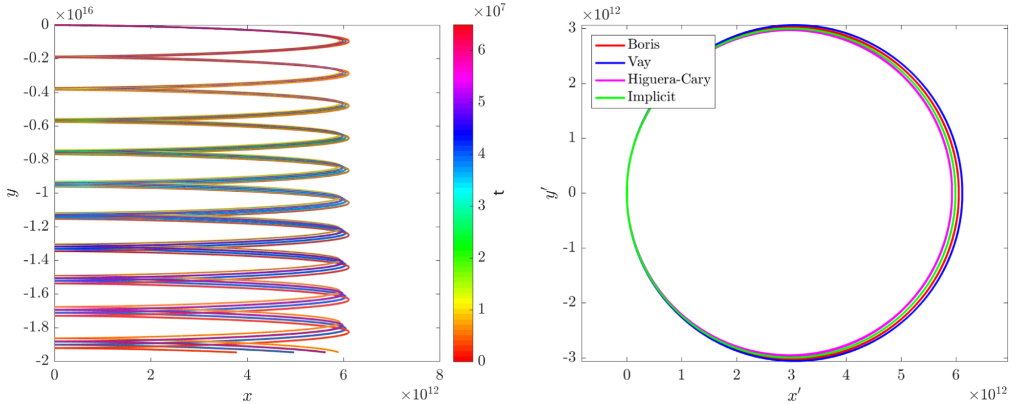
Figure 7. from A Comprehensive Comparison of Relativistic Particle Integrators null 2018 APJS 235 21 doi:10.3847/1538-4365/aab114 https://dx.doi.org/10.3847/1538-4365/aab114 © 2018. The American Astronomical Society. All rights reserved.
