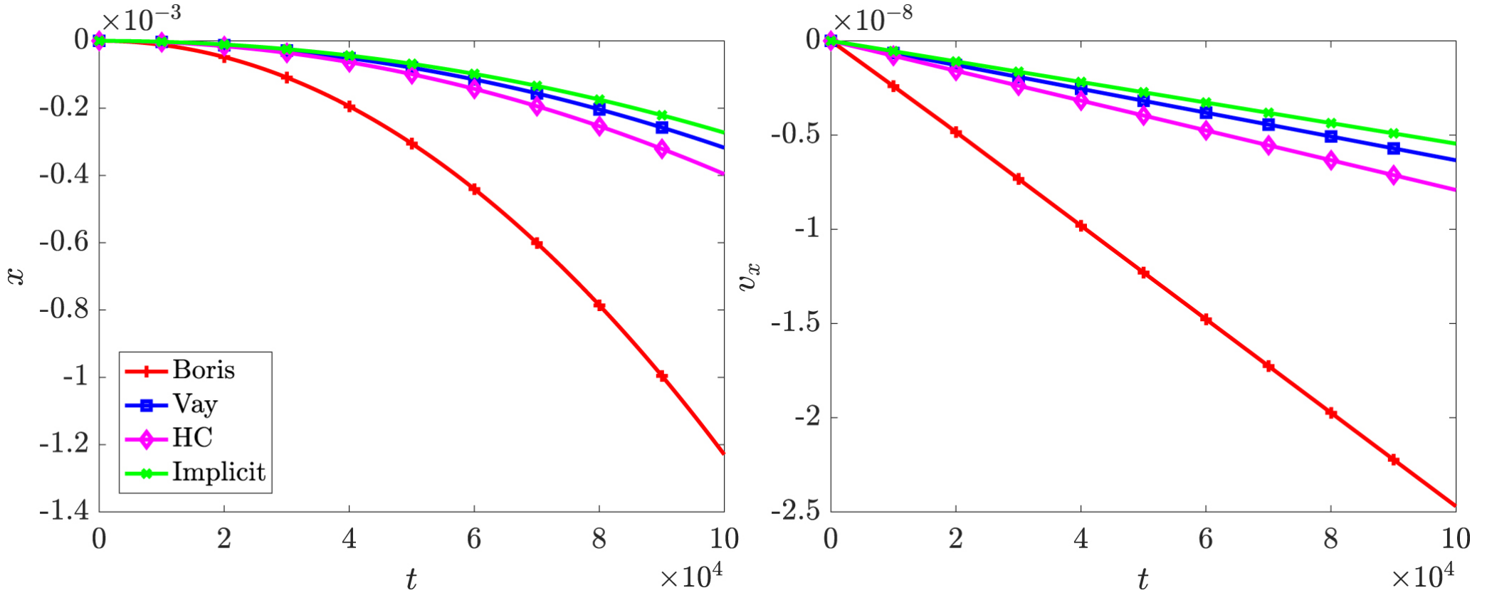
Figure 5. from A Comprehensive Comparison of Relativistic Particle Integrators null 2018 APJS 235 21 doi:10.3847/1538-4365/aab114 https://dx.doi.org/10.3847/1538-4365/aab114 © 2018. The American Astronomical Society. All rights reserved.
