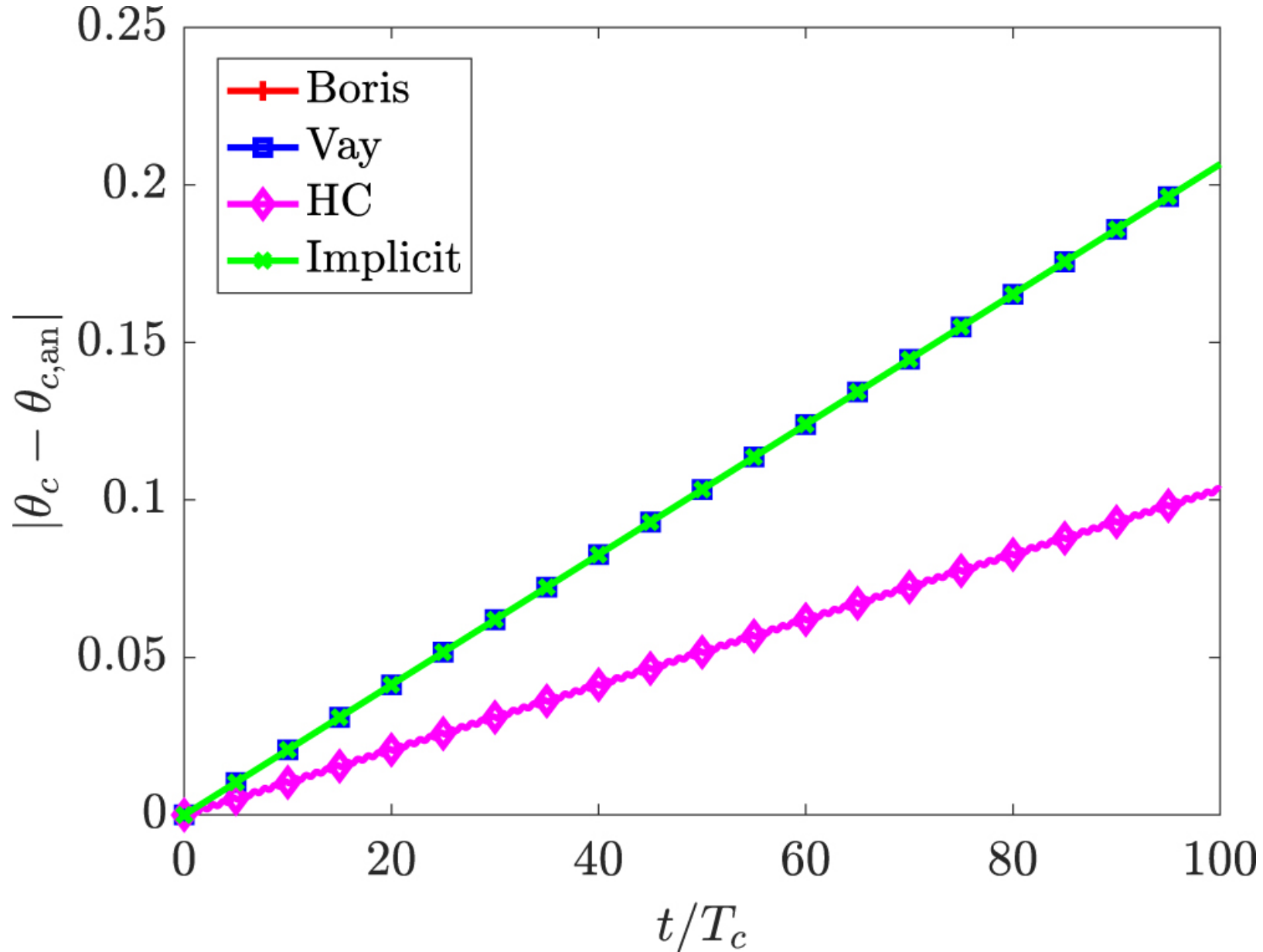
Figure 4. from A Comprehensive Comparison of Relativistic Particle Integrators null 2018 APJS 235 21 doi:10.3847/1538-4365/aab114 https://dx.doi.org/10.3847/1538-4365/aab114 © 2018. The American Astronomical Society. All rights reserved.
