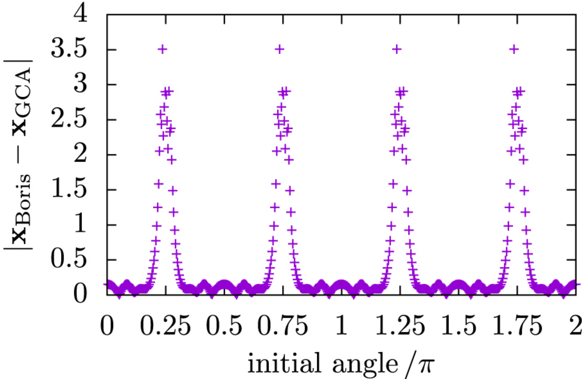
Figure 16. from A Comprehensive Comparison of Relativistic Particle Integrators null 2018 APJS 235 21 doi:10.3847/1538-4365/aab114 https://dx.doi.org/10.3847/1538-4365/aab114 © 2018. The American Astronomical Society. All rights reserved.
