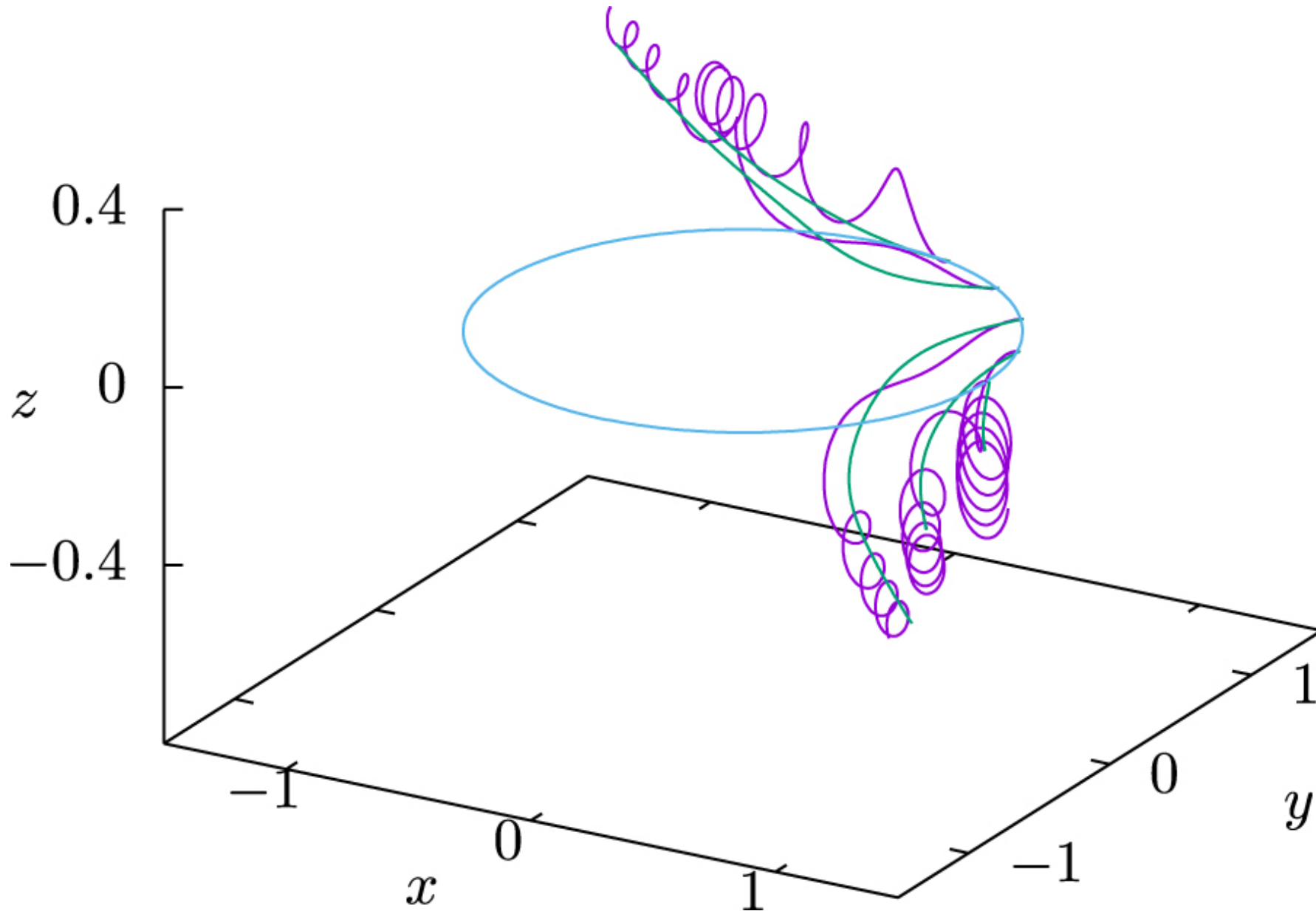
Figure 15. from A Comprehensive Comparison of Relativistic Particle Integrators null 2018 APJS 235 21 doi:10.3847/1538-4365/aab114 https://dx.doi.org/10.3847/1538-4365/aab114 © 2018. The American Astronomical Society. All rights reserved.
