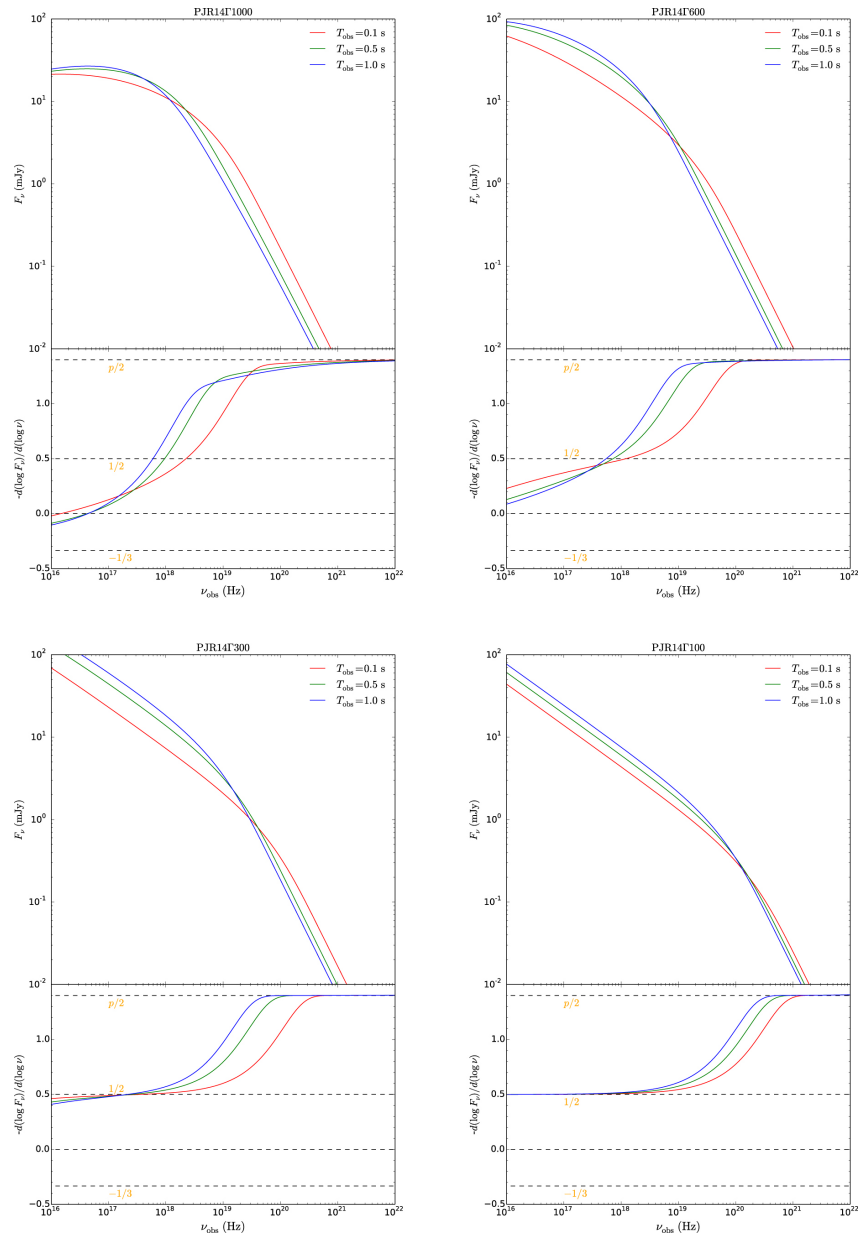
Figure 9. from Low-energy Spectra of Gamma-Ray Bursts from Cooling Electrons null 2018 APJS 234 3 doi:10.3847/1538-4365/aa9e84 https://dx.doi.org/10.3847/1538-4365/aa9e84 © 2018. The American Astronomical Society. All rights reserved.
