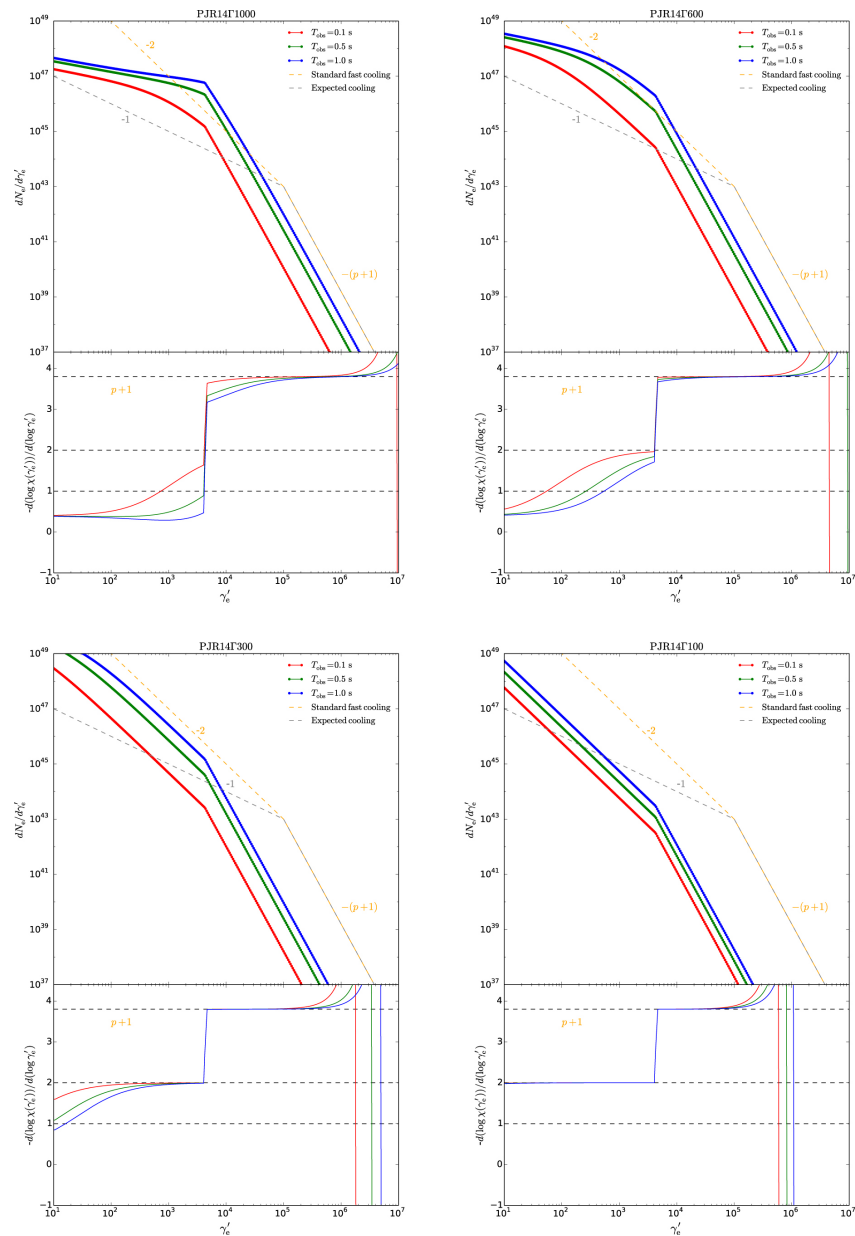
Figure 8. from Low-energy Spectra of Gamma-Ray Bursts from Cooling Electrons null 2018 APJS 234 3 doi:10.3847/1538-4365/aa9e84 https://dx.doi.org/10.3847/1538-4365/aa9e84 © 2018. The American Astronomical Society. All rights reserved.
