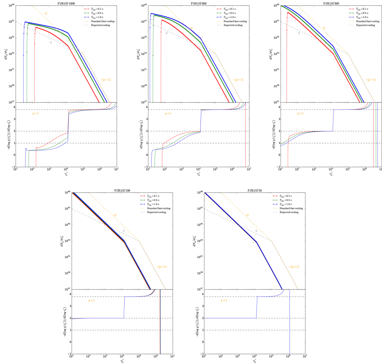
Figure 5. from Low-energy Spectra of Gamma-Ray Bursts from Cooling Electrons null 2018 APJS 234 3 doi:10.3847/1538-4365/aa9e84 https://dx.doi.org/10.3847/1538-4365/aa9e84
