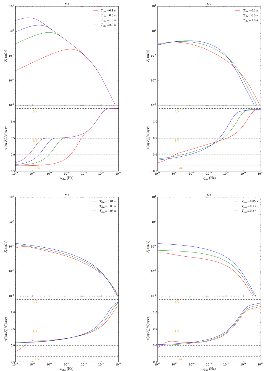
Figure 2. from Low-energy Spectra of Gamma-Ray Bursts from Cooling Electrons null 2018 APJS 234 3 doi:10.3847/1538-4365/aa9e84 https://dx.doi.org/10.3847/1538-4365/aa9e84 © 2018. The American Astronomical Society. All rights reserved.
