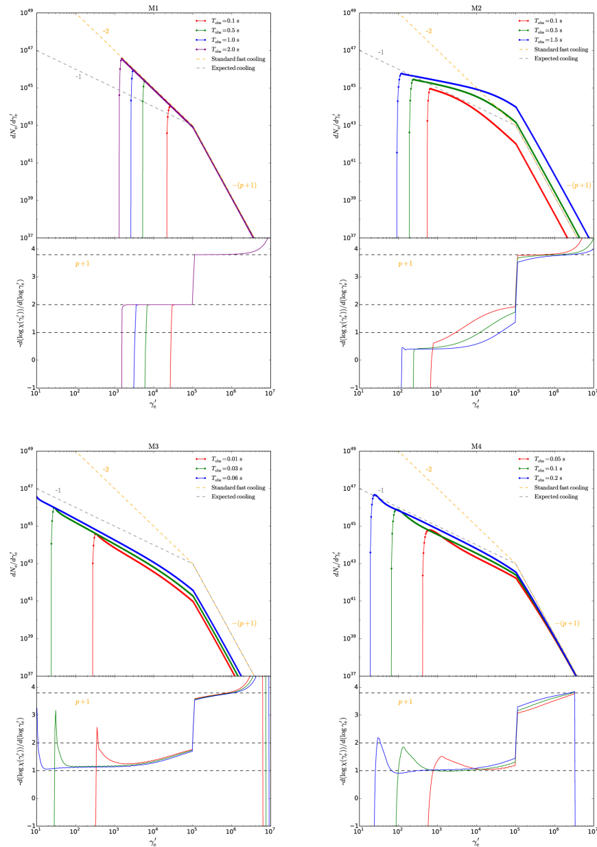
Figure 1. from Low-energy Spectra of Gamma-Ray Bursts from Cooling Electrons null 2018 APJS 234 3 doi:10.3847/1538-4365/aa9e84 https://dx.doi.org/10.3847/1538-4365/aa9e84 © 2018. The American Astronomical Society. All rights reserved.
