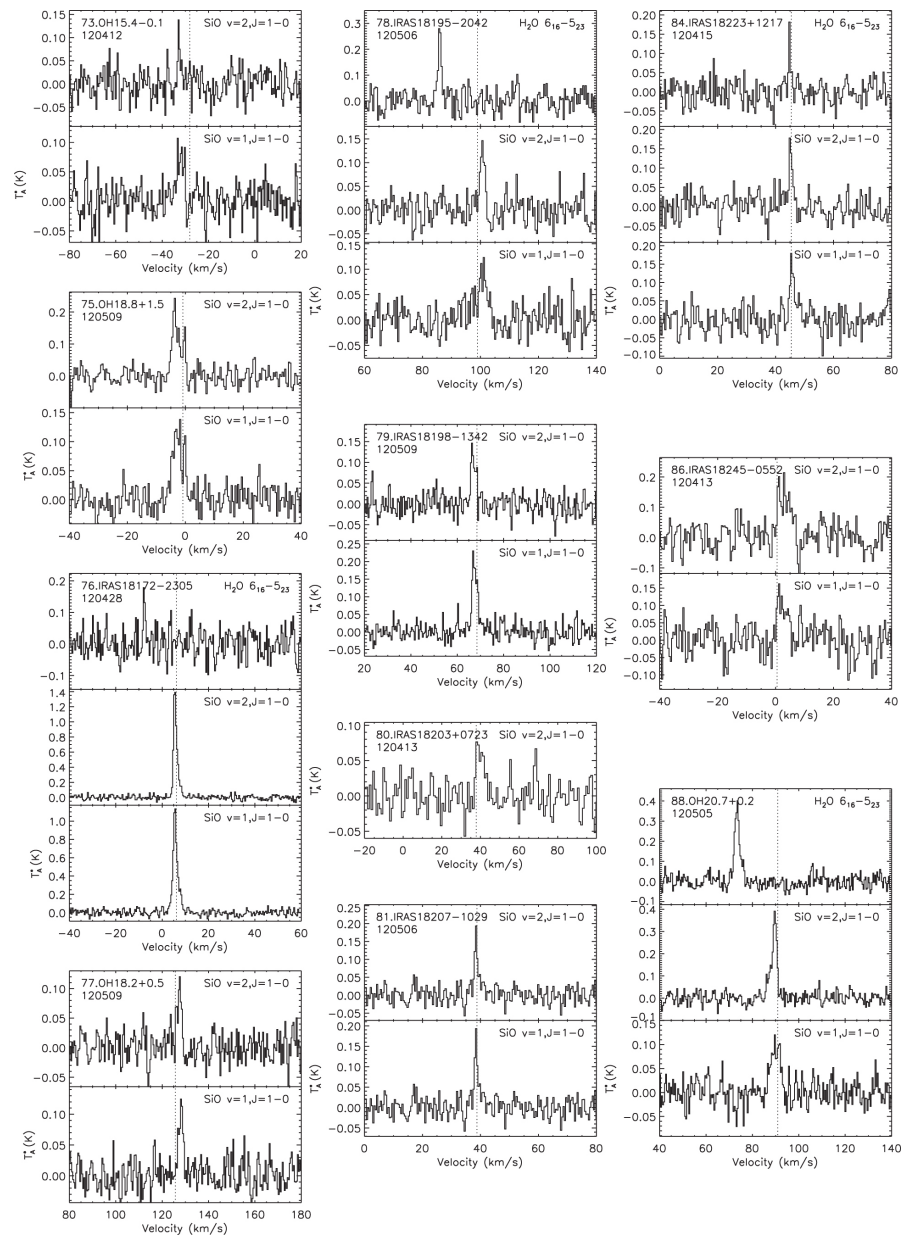
Figure 1. from Simultaneous Observations of H 2 O and SiO Masers toward OH/IR Stars null 2017 APJS 232 13 doi:10.3847/1538-4365/aa85e6 https://dx.doi.org/10.3847/1538-4365/aa85e6
