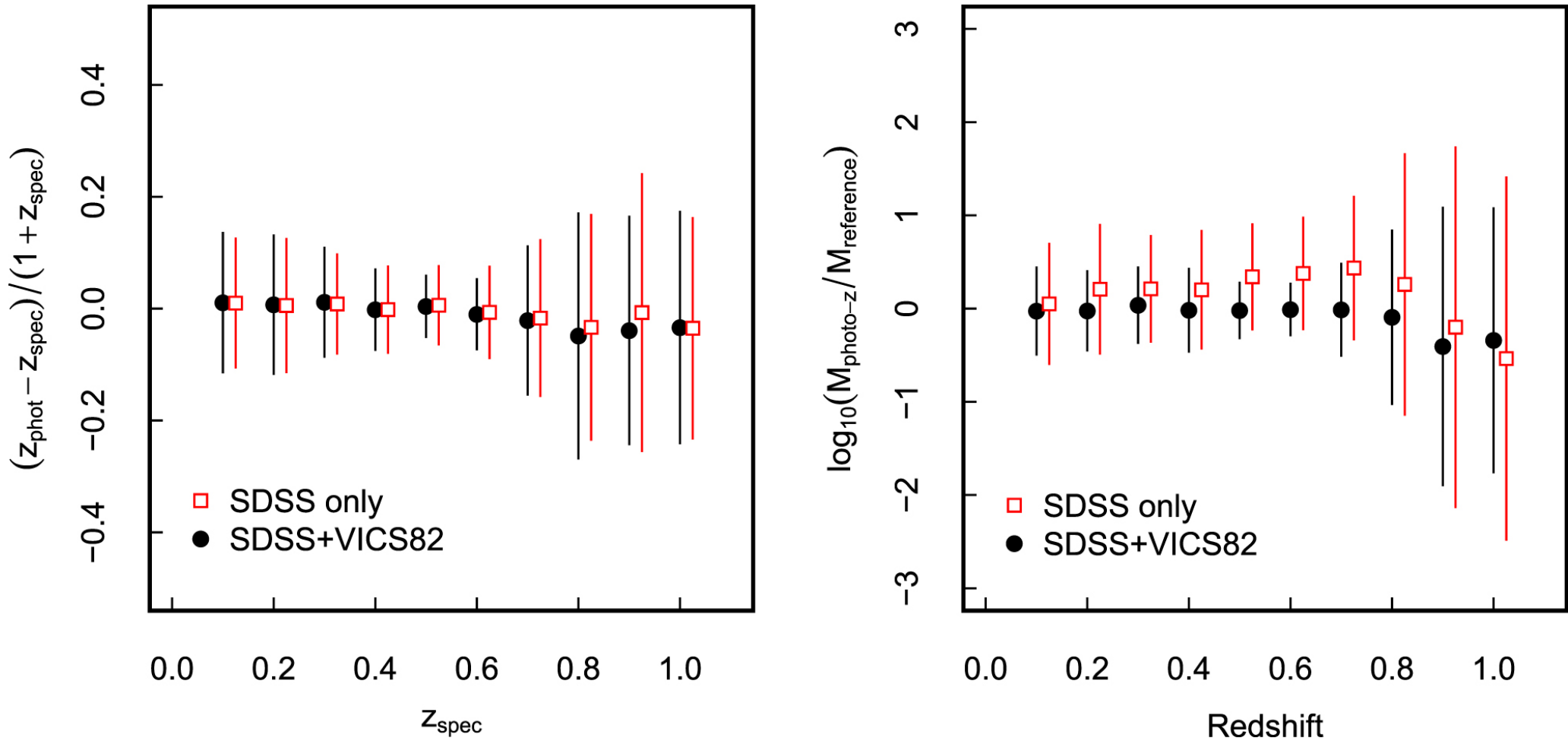
Figure 9. from VICS82: The VISTA–CFHT Stripe 82 Near-infrared Survey null 2017 APJS 231 7 doi:10.3847/1538-4365/aa74b6 https://dx.doi.org/10.3847/1538-4365/aa74b6 © 2017. The American Astronomical Society. All rights reserved.
