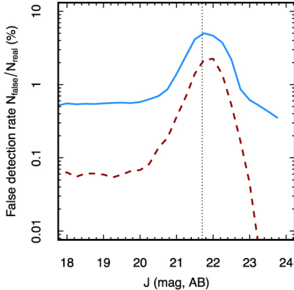
Figure 8. from VICS82: The VISTA–CFHT Stripe 82 Near-infrared Survey null 2017 APJS 231 7 doi:10.3847/1538-4365/aa74b6 https://dx.doi.org/10.3847/1538-4365/aa74b6 © 2017. The American Astronomical Society. All rights reserved.
