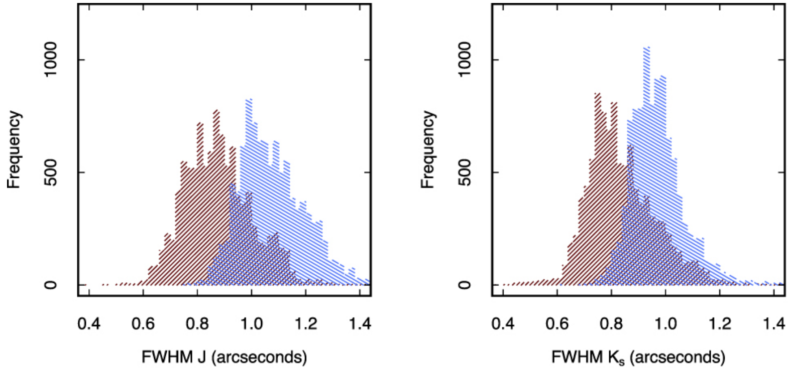
Figure 6. from VICS82: The VISTA–CFHT Stripe 82 Near-infrared Survey null 2017 APJS 231 7 doi:10.3847/1538-4365/aa74b6 https://dx.doi.org/10.3847/1538-4365/aa74b6 © 2017. The American Astronomical Society. All rights reserved.
