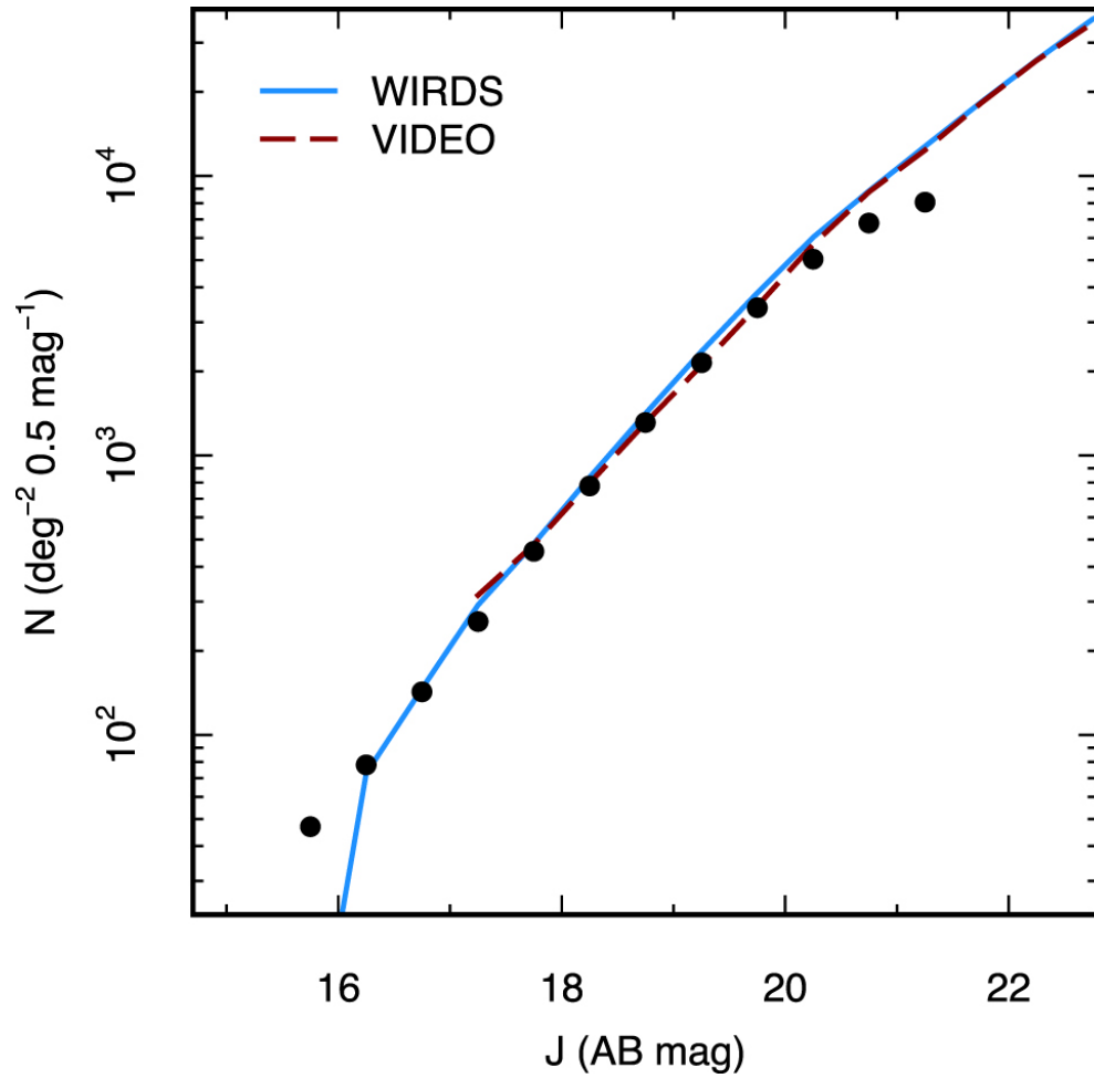
Figure 5. from VICS82: The VISTA–CFHT Stripe 82 Near-infrared Survey null 2017 APJS 231 7 doi:10.3847/1538-4365/aa74b6 https://dx.doi.org/10.3847/1538-4365/aa74b6 © 2017. The American Astronomical Society. All rights reserved.
