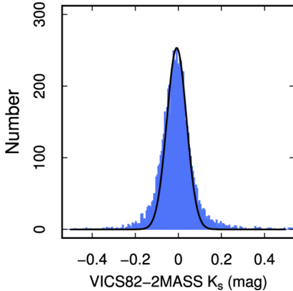
Figure 4. from VICS82: The VISTA–CFHT Stripe 82 Near-infrared Survey null 2017 APJS 231 7 doi:10.3847/1538-4365/aa74b6 https://dx.doi.org/10.3847/1538-4365/aa74b6 © 2017. The American Astronomical Society. All rights reserved.
