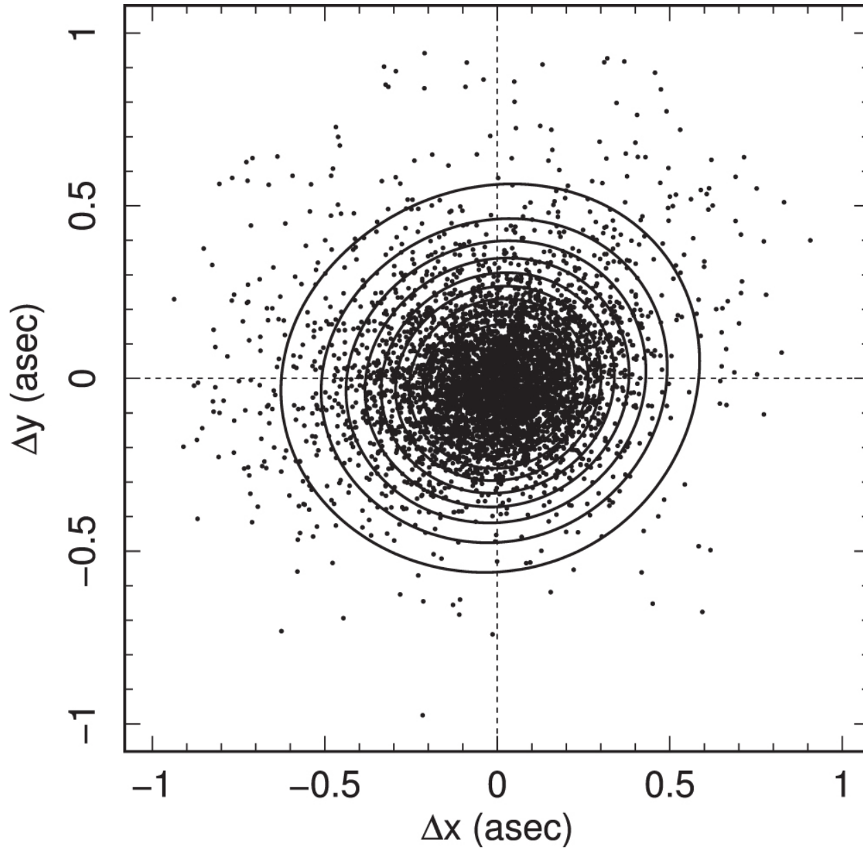
Figure 3. from VICS82: The VISTA–CFHT Stripe 82 Near-infrared Survey null 2017 APJS 231 7 doi:10.3847/1538-4365/aa74b6 https://dx.doi.org/10.3847/1538-4365/aa74b6 © 2017. The American Astronomical Society. All rights reserved.
