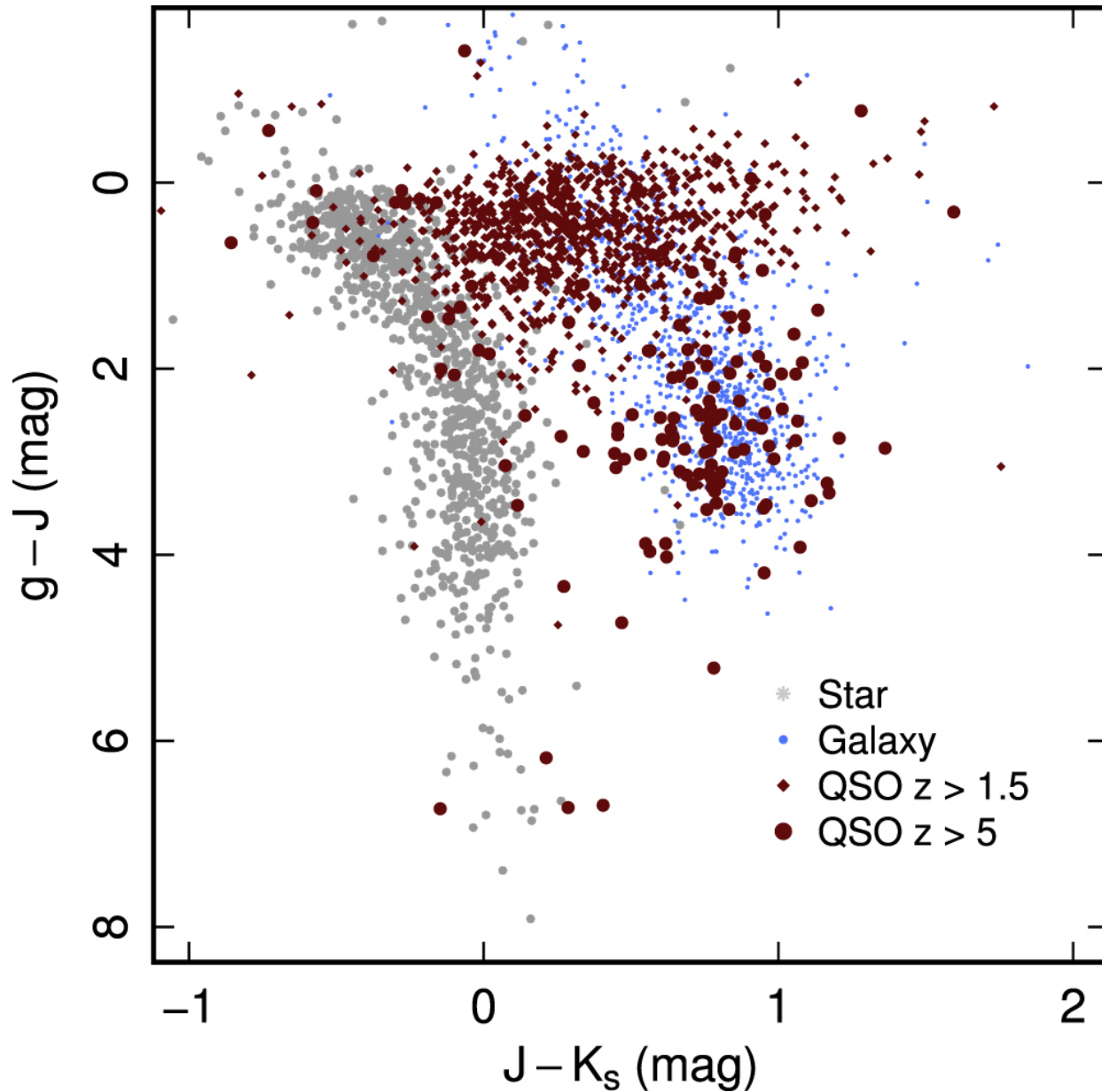
Figure 11. from VICS82: The VISTA–CFHT Stripe 82 Near-infrared Survey null 2017 APJS 231 7 doi:10.3847/1538-4365/aa74b6 https://dx.doi.org/10.3847/1538-4365/aa74b6 © 2017. The American Astronomical Society. All rights reserved.
