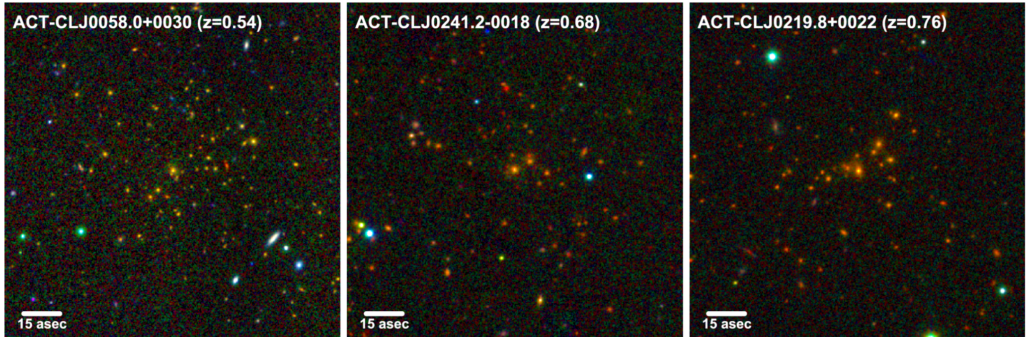
Figure 10. from VICS82: The VISTA–CFHT Stripe 82 Near-infrared Survey null 2017 APJS 231 7 doi:10.3847/1538-4365/aa74b6 https://dx.doi.org/10.3847/1538-4365/aa74b6 © 2017. The American Astronomical Society. All rights reserved.
