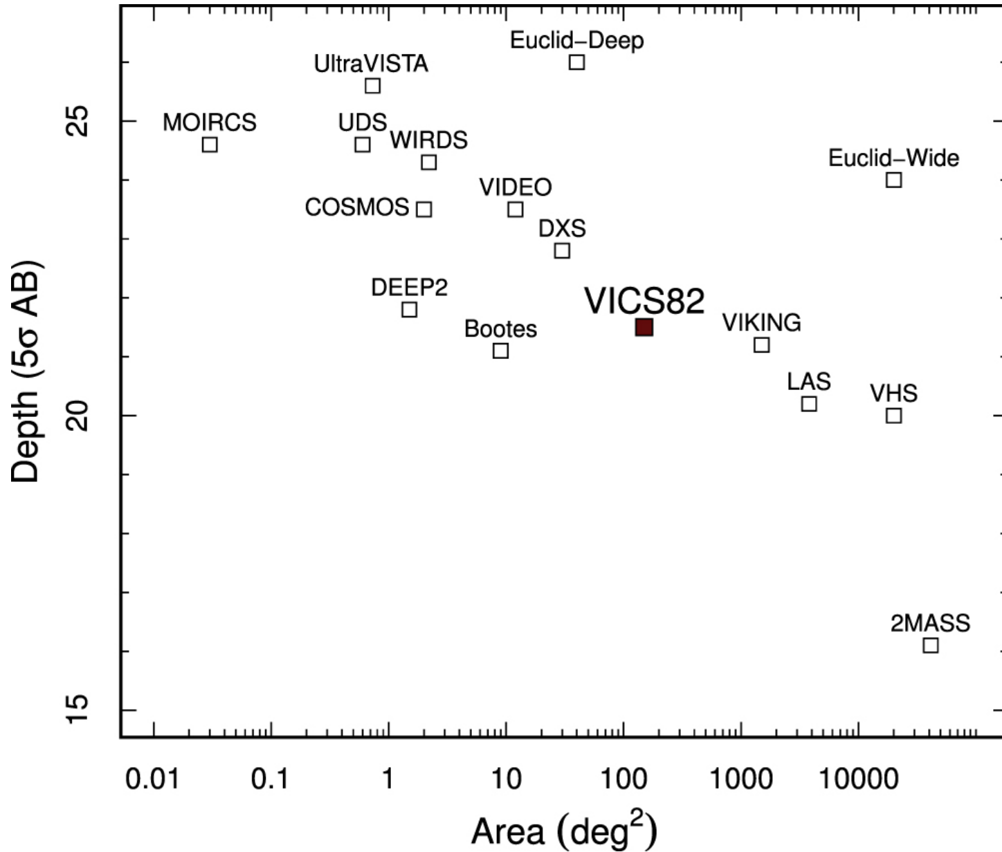
Figure 1. from VICS82: The VISTA–CFHT Stripe 82 Near-infrared Survey null 2017 APJS 231 7 doi:10.3847/1538-4365/aa74b6 https://dx.doi.org/10.3847/1538-4365/aa74b6 © 2017. The American Astronomical Society. All rights reserved.
