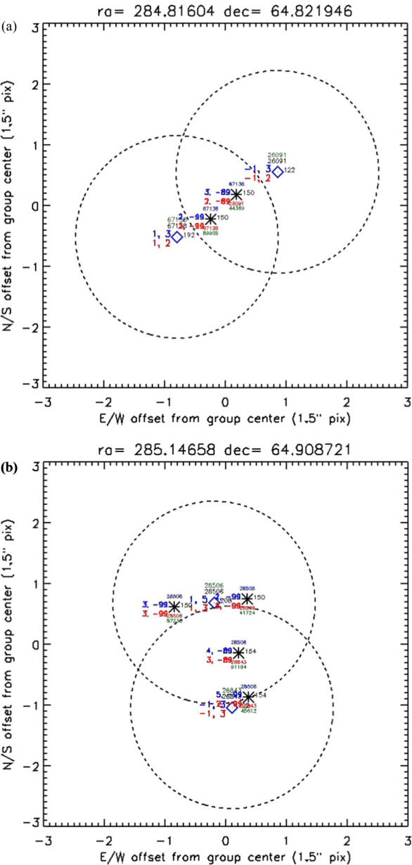
Figure 7. from Revised Catalog of GALEX Ultraviolet Sources. I. The All-Sky Survey: GUVcat_AIS null 2017 APJS 230 24 doi:10.3847/1538-4365/aa7053 https://dx.doi.org/10.3847/1538-4365/aa7053 © 2017. The American Astronomical Society. All rights reserved.
