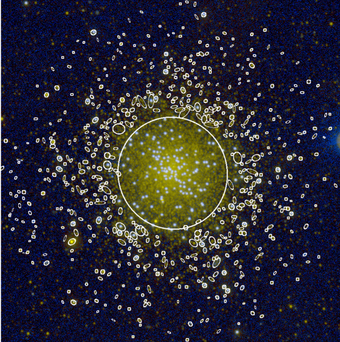
Figure 5. from Revised Catalog of GALEX Ultraviolet Sources. I. The All-Sky Survey: GUVcat_AIS null 2017 APJS 230 24 doi:10.3847/1538-4365/aa7053 https://dx.doi.org/10.3847/1538-4365/aa7053 © 2017. The American Astronomical Society. All rights reserved.
