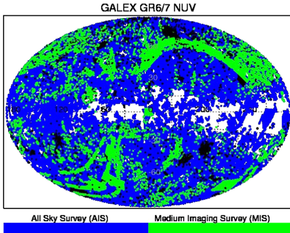
Figure 1. from Revised Catalog of GALEX Ultraviolet Sources. I. The All-Sky Survey: GUVcat_AIS null 2017 APJS 230 24 doi:10.3847/1538-4365/aa7053 https://dx.doi.org/10.3847/1538-4365/aa7053 © 2017. The American Astronomical Society. All rights reserved.
