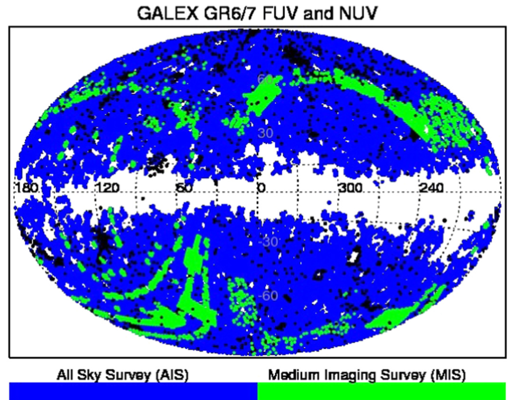
Figure 1. from Revised Catalog of GALEX Ultraviolet Sources. I. The All-Sky Survey: GUVcat_AIS null 2017 APJS 230 24 doi:10.3847/1538-4365/aa7053 https://dx.doi.org/10.3847/1538-4365/aa7053 © 2017. The American Astronomical Society. All rights reserved.
