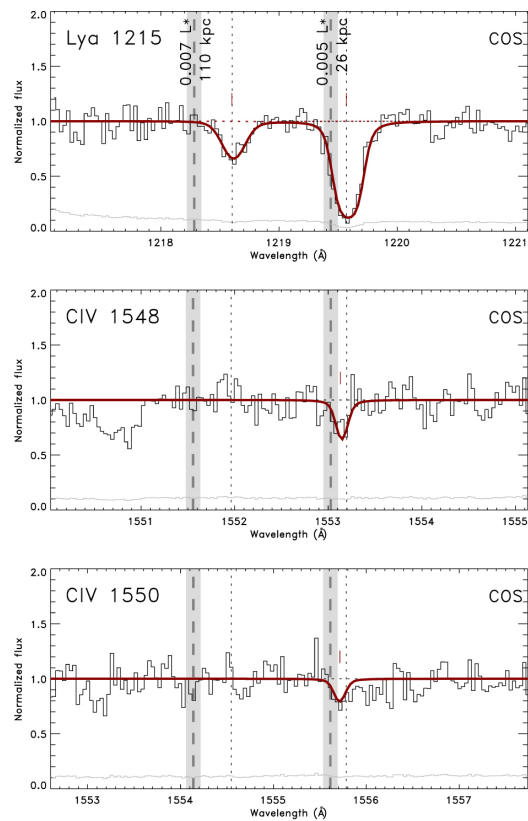
4.1: IES 1028+511 absorbers at cz_{\text{abs}} = 728 & 967 \text{ km s}^{-1} (Systems 1 & 2).
