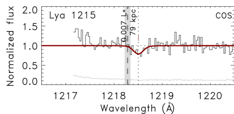
4.2: ISAX J1032.3+5051 absorber at cz_{\text{abs}} = 704 \text{ km s}^{-1} (System 3).
