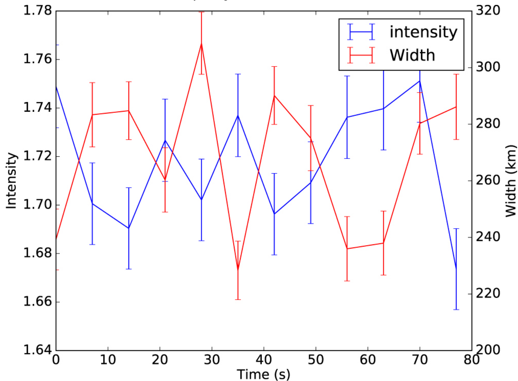
Figure 7. from Oscillations on Width and Intensity of Slender Ca II H Fibrils from SUNRISE/SuFI null 2017 APJS 229 7 doi:10.3847/1538-4365/229/1/7 https://dx.doi.org/10.3847/1538-4365/229/1/7 © 2017. The American Astronomical Society. All rights reserved.
