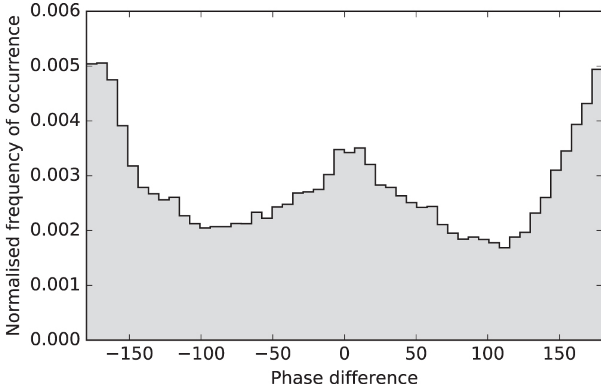
Figure 6. from Oscillations on Width and Intensity of Slender Ca II H Fibrils from SUNRISE/SuFI null 2017 APJS 229 7 doi:10.3847/1538-4365/229/1/7 https://dx.doi.org/10.3847/1538-4365/229/1/7 © 2017. The American Astronomical Society. All rights reserved.
