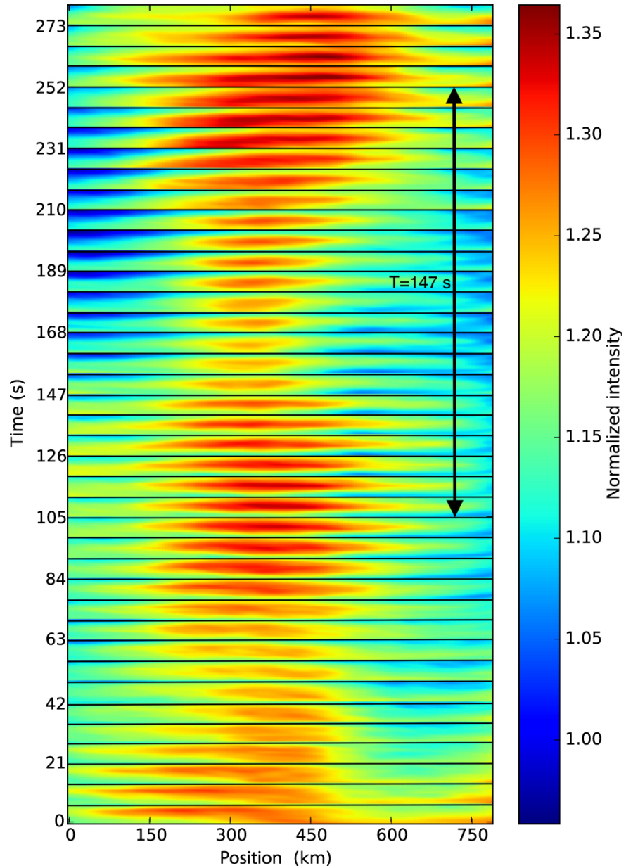
Figure 3. from Oscillations on Width and Intensity of Slender Ca II H Fibrils from SUNRISE/SuFI null 2017 APJS 229 7 doi:10.3847/1538-4365/229/1/7 https://dx.doi.org/10.3847/1538-4365/229/1/7
