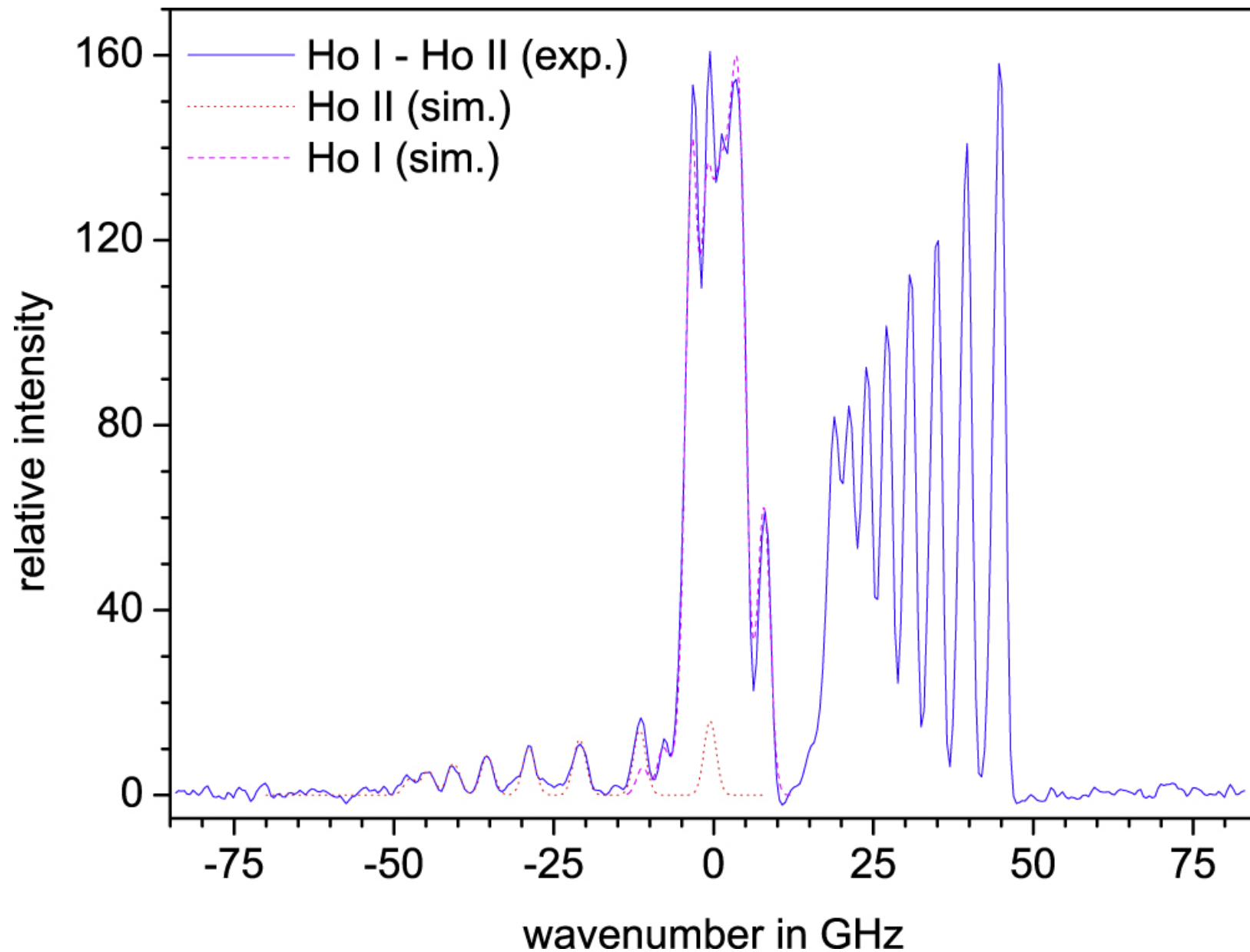
Figure 5. from Line Identification of Atomic and Ionic Spectra of Holmium in the Near-UV. Part I. Spectrum of Ho I null 2017 APJS 228 16 doi:10.3847/1538-4365/228/2/16 https://dx.doi.org/10.3847/1538-4365/228/2/16 © 2017. The American Astronomical Society. All rights reserved.
