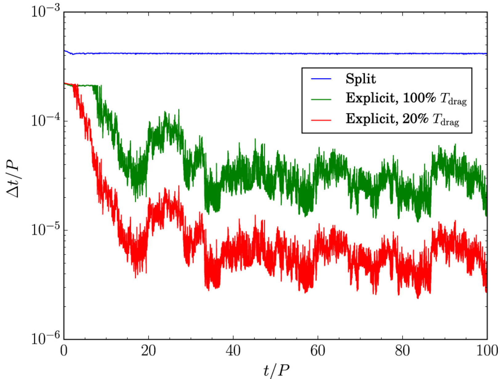
Figure 15. from INTEGRATION OF PARTICLE-GAS SYSTEMS WITH STIFF MUTUAL DRAG INTERACTION null 2016 APJS 224 39 doi:10.3847/0067-0049/224/2/39 https://dx.doi.org/10.3847/0067-0049/224/2/39 © 2016. The American Astronomical Society. All rights reserved.
