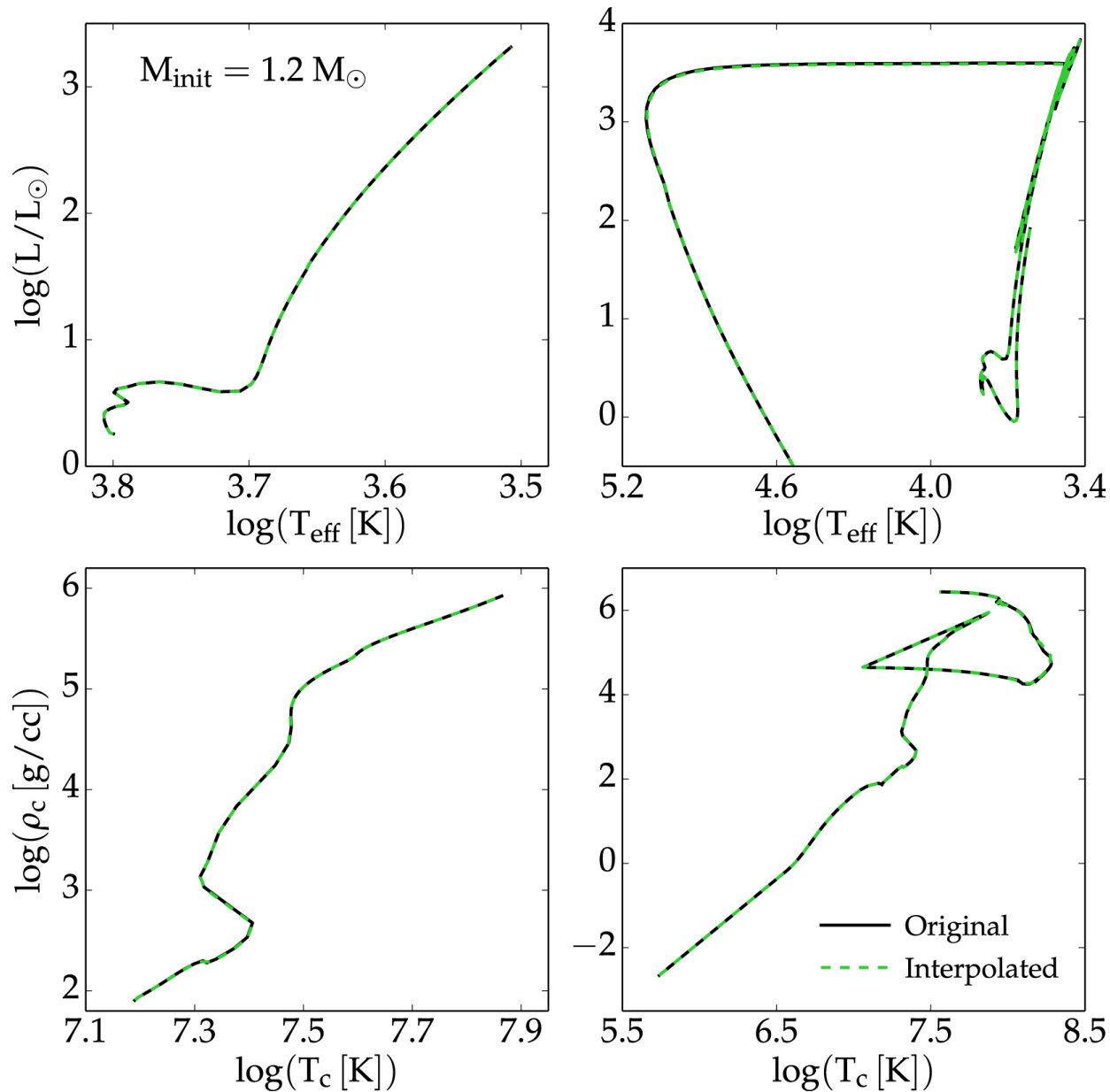
Figure 9. from MESA ISOCHRONES AND STELLAR TRACKS (MIST) 0: METHODS FOR THE CONSTRUCTION OF STELLAR ISOCHRONES null 2016 APJS 222 8 doi:10.3847/0067-0049/222/1/8 https://dx.doi.org/10.3847/0067-0049/222/1/8 © 2016. The American Astronomical Society. All rights reserved.
