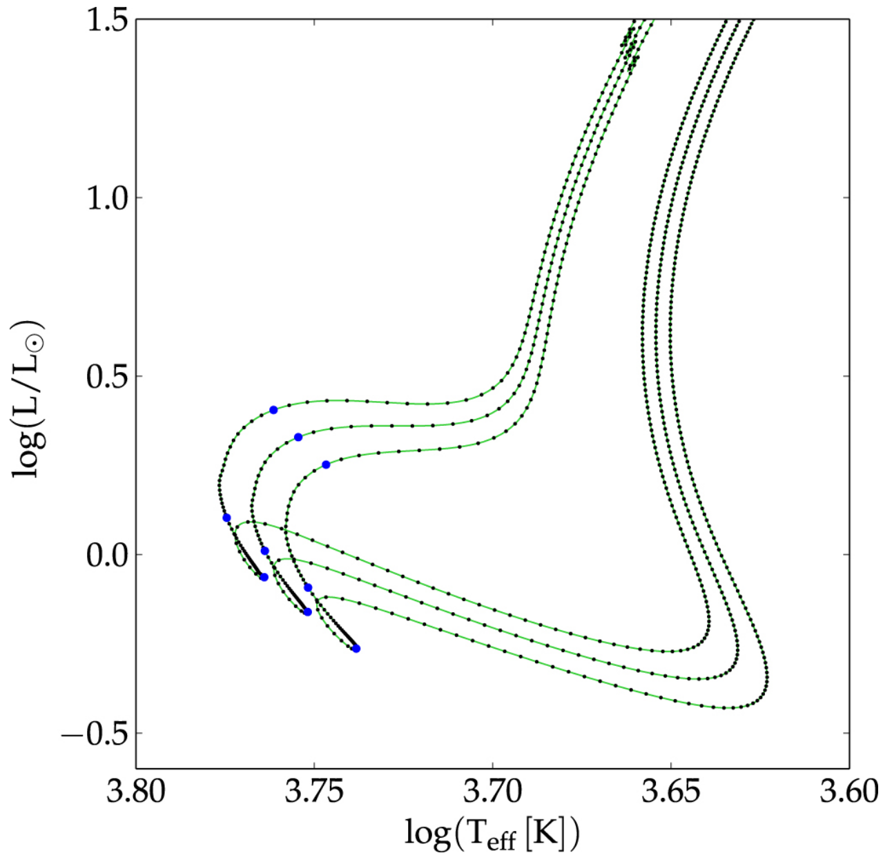
Figure 8. from MESA ISOCHRONES AND STELLAR TRACKS (MIST) 0: METHODS FOR THE CONSTRUCTION OF STELLAR ISOCHRONES null 2016 APJS 222 8 doi:10.3847/0067-0049/222/1/8 https://dx.doi.org/10.3847/0067-0049/222/1/8 © 2016. The American Astronomical Society. All rights reserved.
