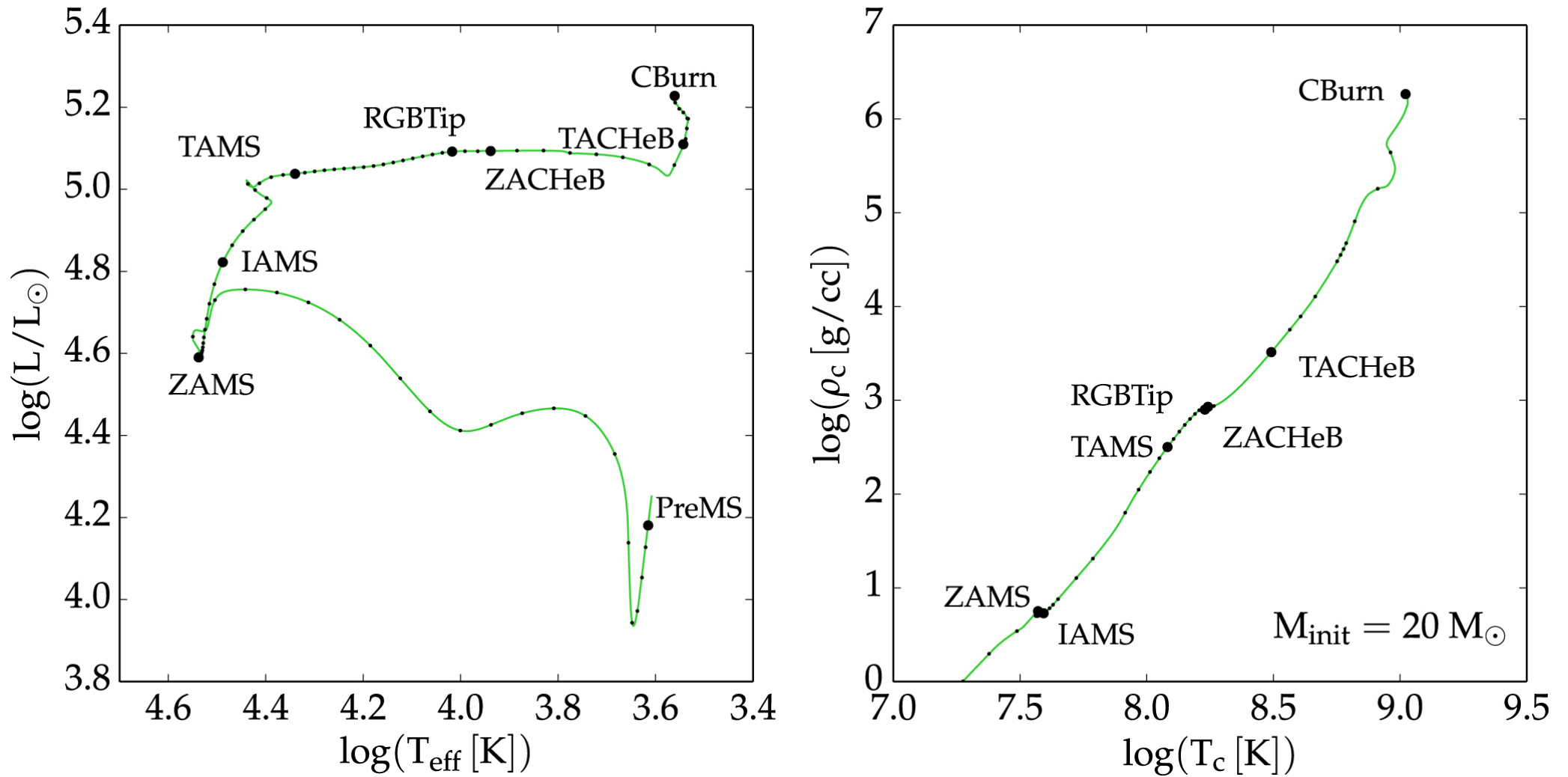
Figure 7. from MESA ISOCHRONES AND STELLAR TRACKS (MIST) 0: METHODS FOR THE CONSTRUCTION OF STELLAR ISOCHRONES null 2016 APJS 222 8 doi:10.3847/0067-0049/222/1/8 https://dx.doi.org/10.3847/0067-0049/222/1/8 © 2016. The American Astronomical Society. All rights reserved.
