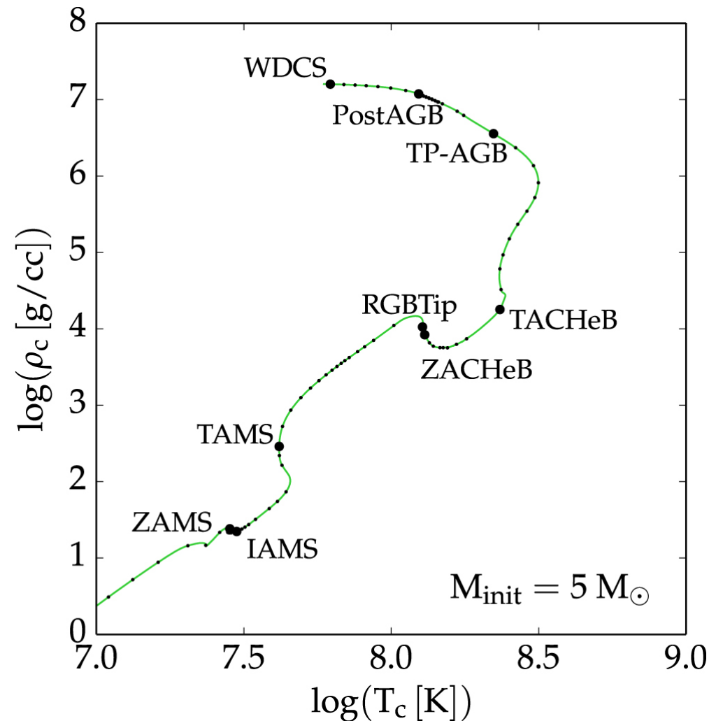
Figure 6. from MESA ISOCHRONES AND STELLAR TRACKS (MIST) 0: METHODS FOR THE CONSTRUCTION OF STELLAR ISOCHRONES null 2016 APJS 222 8 doi:10.3847/0067-0049/222/1/8 https://dx.doi.org/10.3847/0067-0049/222/1/8 © 2016. The American Astronomical Society. All rights reserved.
