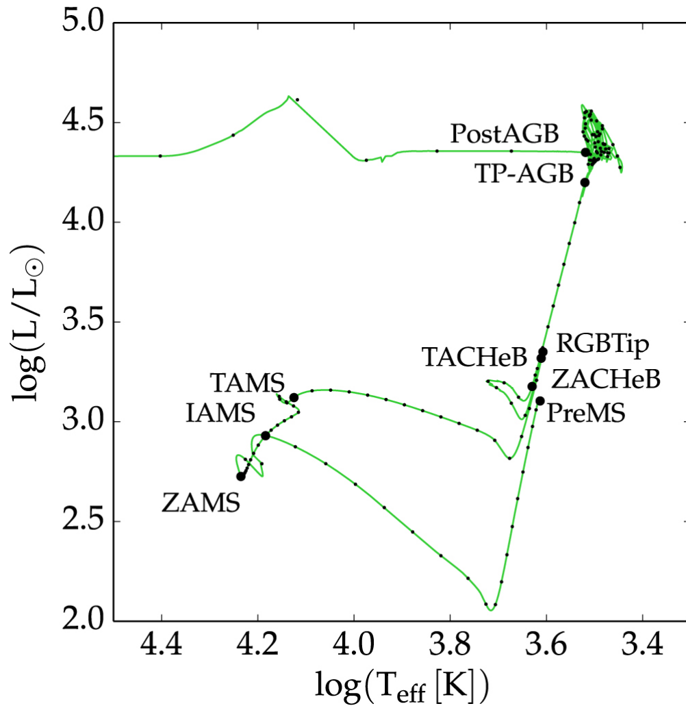
Figure 6. from MESA ISOCHRONES AND STELLAR TRACKS (MIST) 0: METHODS FOR THE CONSTRUCTION OF STELLAR ISOCHRONES null 2016 APJS 222 8 doi:10.3847/0067-0049/222/1/8 https://dx.doi.org/10.3847/0067-0049/222/1/8 © 2016. The American Astronomical Society. All rights reserved.
