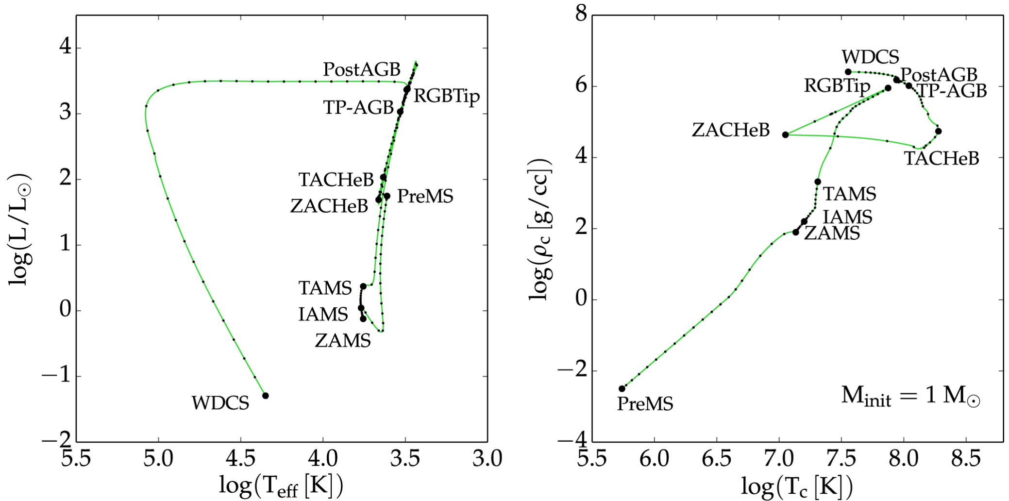
Figure 5. from MESA ISOCHRONES AND STELLAR TRACKS (MIST) 0: METHODS FOR THE CONSTRUCTION OF STELLAR ISOCHRONES null 2016 APJS 222 8 doi:10.3847/0067-0049/222/1/8 https://dx.doi.org/10.3847/0067-0049/222/1/8 © 2016. The American Astronomical Society. All rights reserved.
