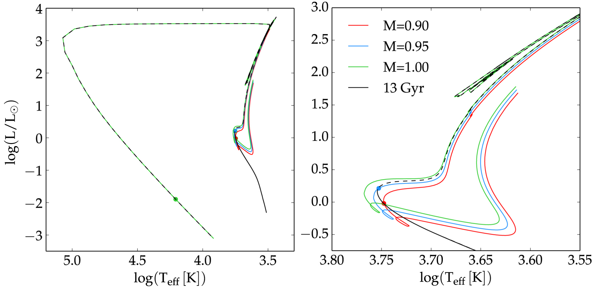
Figure 3. from MESA ISOCHRONES AND STELLAR TRACKS (MIST) 0: METHODS FOR THE CONSTRUCTION OF STELLAR ISOCHRONES null 2016 APJS 222 8 doi:10.3847/0067-0049/222/1/8 https://dx.doi.org/10.3847/0067-0049/222/1/8 © 2016. The American Astronomical Society. All rights reserved.
