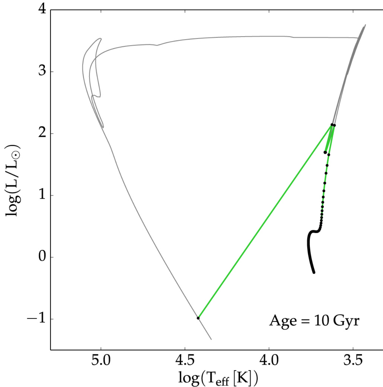
Figure 2. from MESA ISOCHRONES AND STELLAR TRACKS (MIST) 0: METHODS FOR THE CONSTRUCTION OF STELLAR ISOCHRONES null 2016 APJS 222 8 doi:10.3847/0067-0049/222/1/8 https://dx.doi.org/10.3847/0067-0049/222/1/8 © 2016. The American Astronomical Society. All rights reserved.
