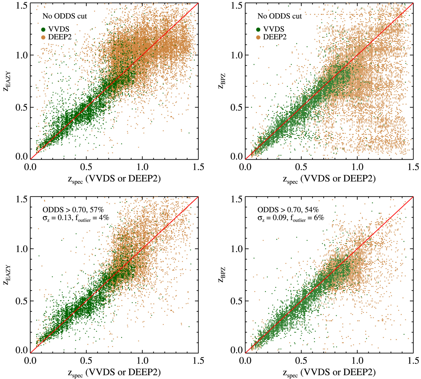
Figure 8. from THE STRIPE 82 MASSIVE GALAXY PROJECT. I. CATALOG CONSTRUCTION null 2015 APJS 221 15 doi:10.1088/0067-0049/221/1/15 https://dx.doi.org/10.1088/0067-0049/221/1/15
