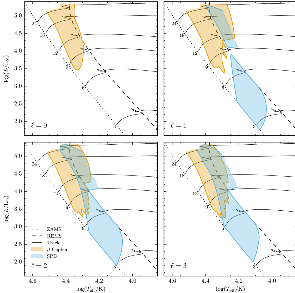
Figure 9. from MODULES FOR EXPERIMENTS IN STELLAR ASTROPHYSICS (MESA): BINARIES, PULSATIONS, AND EXPLOSIONS null 2015 APJS 220 15 doi:10.1088/0067-0049/220/1/15 https://dx.doi.org/10.1088/0067-0049/220/1/15 © 2015. The American Astronomical Society. All rights reserved.
