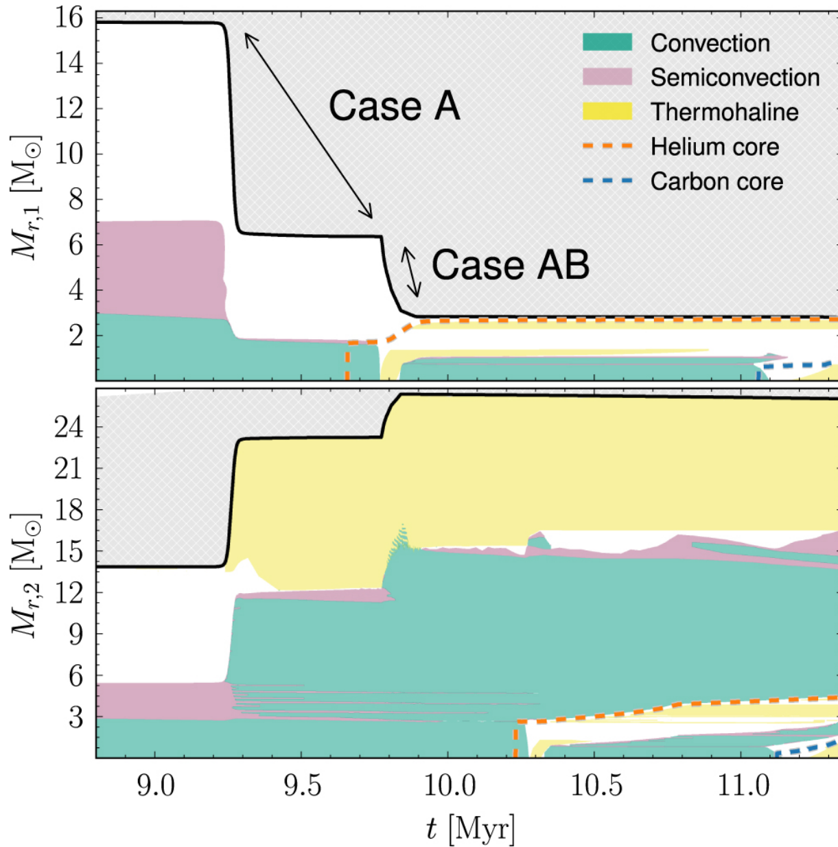
Figure 7. from MODULES FOR EXPERIMENTS IN STELLAR ASTROPHYSICS (MESA): BINARIES, PULSATIONS, AND EXPLOSIONS null 2015 APJS 220 15 doi:10.1088/0067-0049/220/1/15 https://dx.doi.org/10.1088/0067-0049/220/1/15 © 2015. The American Astronomical Society. All rights reserved.
