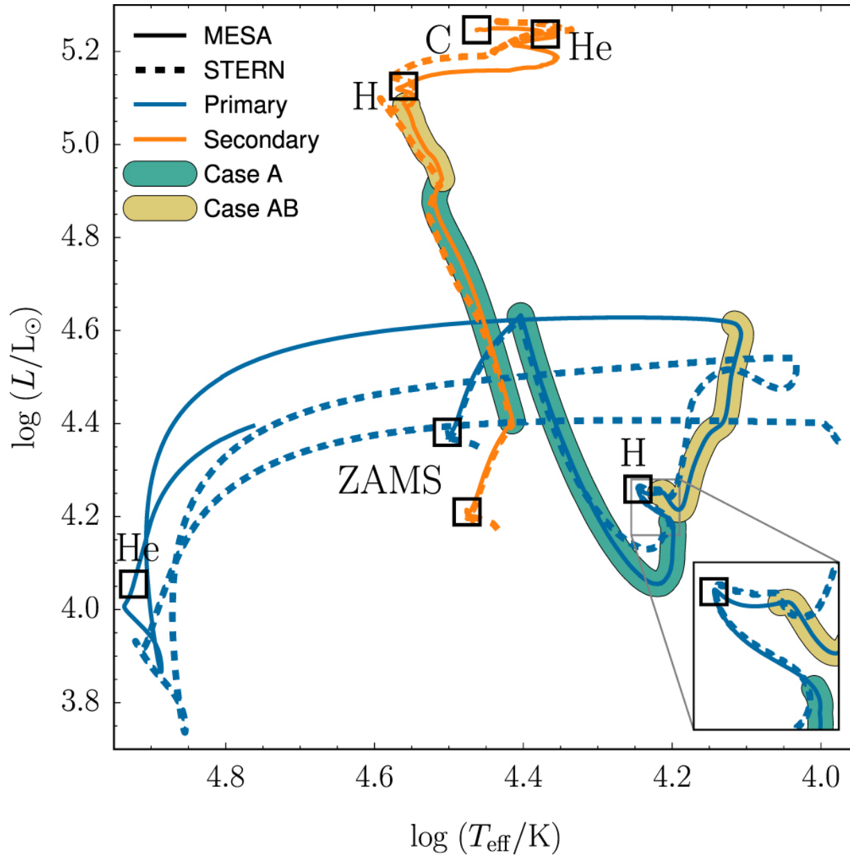
Figure 6. from MODULES FOR EXPERIMENTS IN STELLAR ASTROPHYSICS (MESA): BINARIES, PULSATIONS, AND EXPLOSIONS null 2015 APJS 220 15 doi:10.1088/0067-0049/220/1/15 https://dx.doi.org/10.1088/0067-0049/220/1/15 © 2015. The American Astronomical Society. All rights reserved.
