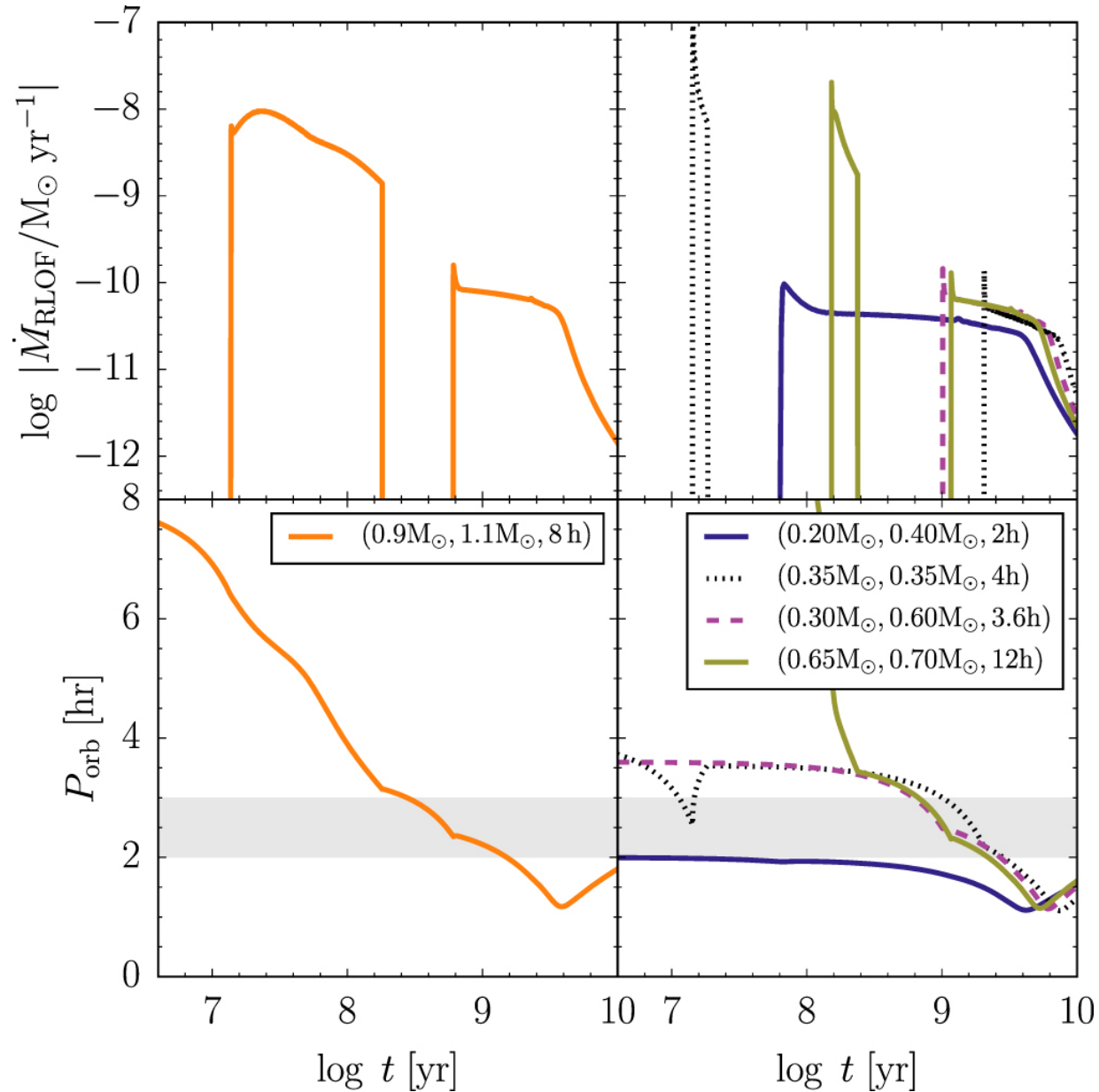
Figure 5. from MODULES FOR EXPERIMENTS IN STELLAR ASTROPHYSICS (MESA): BINARIES, PULSATIONS, AND EXPLOSIONS null 2015 APJS 220 15 doi:10.1088/0067-0049/220/1/15 https://dx.doi.org/10.1088/0067-0049/220/1/15 © 2015. The American Astronomical Society. All rights reserved.
