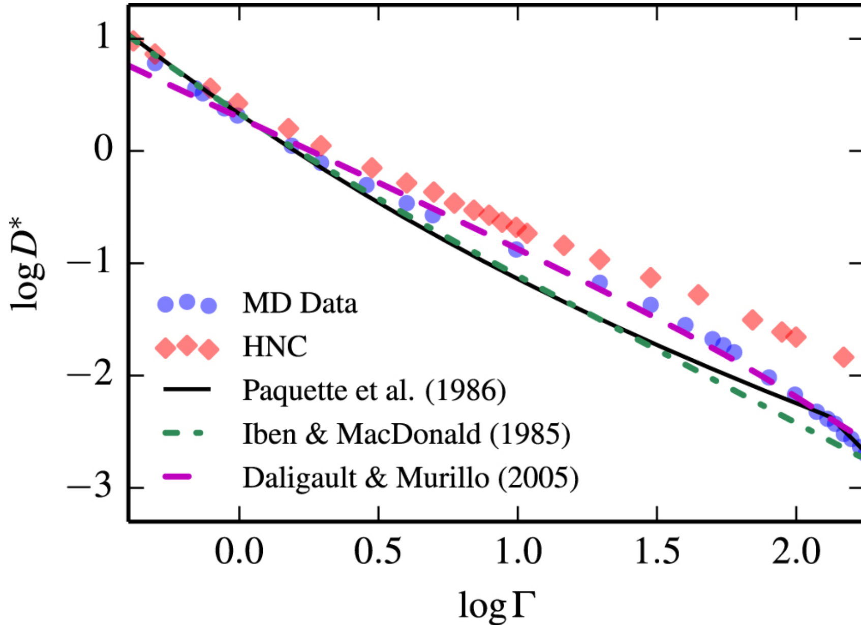
Figure 44. from MODULES FOR EXPERIMENTS IN STELLAR ASTROPHYSICS (MESA): BINARIES, PULSATIONS, AND EXPLOSIONS null 2015 APJS 220 15 doi:10.1088/0067-0049/220/1/15 https://dx.doi.org/10.1088/0067-0049/220/1/15 © 2015. The American Astronomical Society. All rights reserved.
