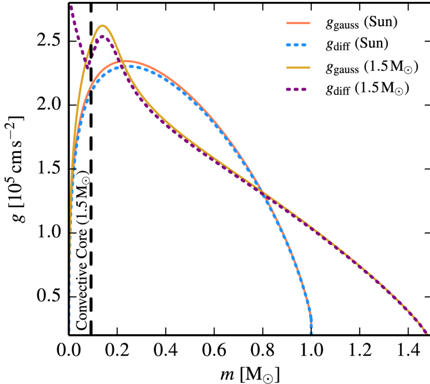
Figure 41. from MODULES FOR EXPERIMENTS IN STELLAR ASTROPHYSICS (MESA): BINARIES, PULSATIONS, AND EXPLOSIONS null 2015 APJS 220 15 doi:10.1088/0067-0049/220/1/15 https://dx.doi.org/10.1088/0067-0049/220/1/15 © 2015. The American Astronomical Society. All rights reserved.
