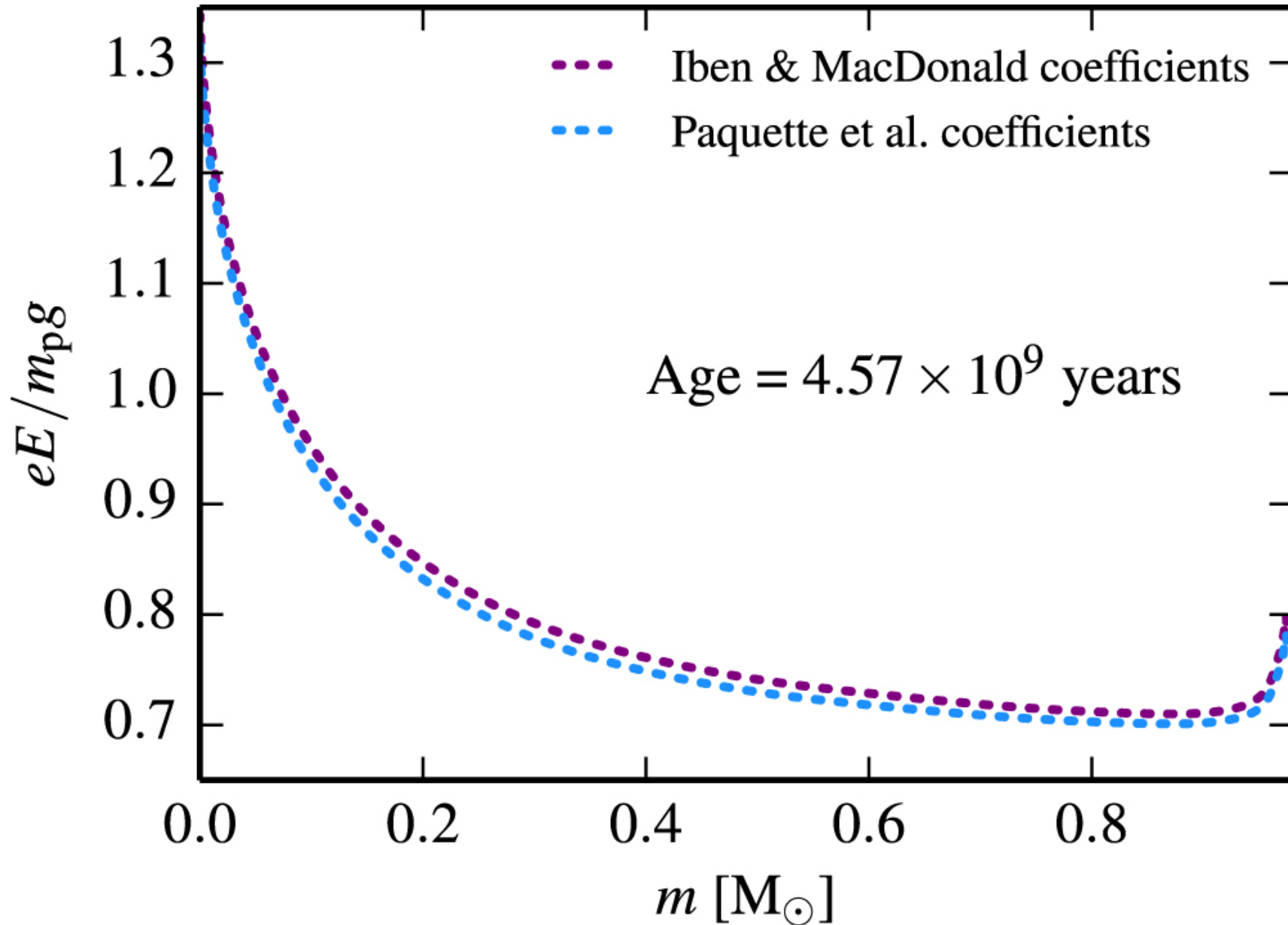
Figure 40. from MODULES FOR EXPERIMENTS IN STELLAR ASTROPHYSICS (MESA): BINARIES, PULSATIONS, AND EXPLOSIONS null 2015 APJS 220 15 doi:10.1088/0067-0049/220/1/15 https://dx.doi.org/10.1088/0067-0049/220/1/15 © 2015. The American Astronomical Society. All rights reserved.
