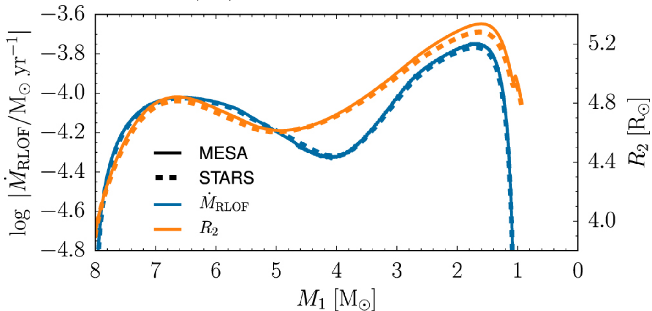
Figure 4. from MODULES FOR EXPERIMENTS IN STELLAR ASTROPHYSICS (MESA): BINARIES, PULSATIONS, AND EXPLOSIONS null 2015 APJS 220 15 doi:10.1088/0067-0049/220/1/15 https://dx.doi.org/10.1088/0067-0049/220/1/15 © 2015. The American Astronomical Society. All rights reserved.
