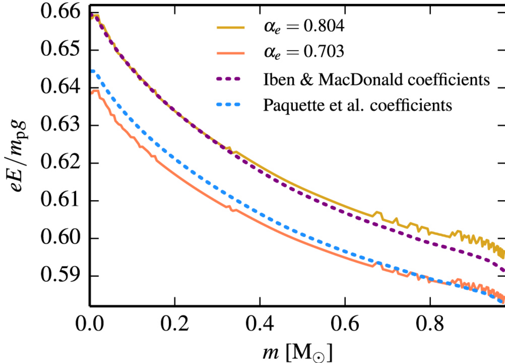
Figure 39. from MODULES FOR EXPERIMENTS IN STELLAR ASTROPHYSICS (MESA): BINARIES, PULSATIONS, AND EXPLOSIONS null 2015 APJS 220 15 doi:10.1088/0067-0049/220/1/15 https://dx.doi.org/10.1088/0067-0049/220/1/15 © 2015. The American Astronomical Society. All rights reserved.
