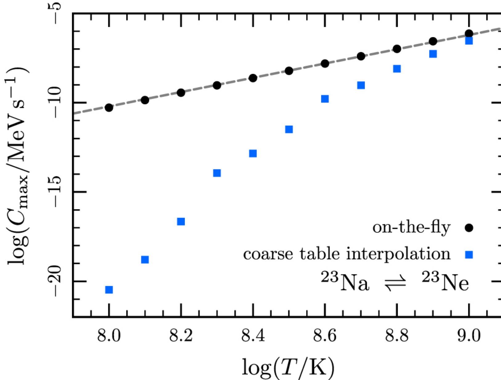
Figure 36. from MODULES FOR EXPERIMENTS IN STELLAR ASTROPHYSICS (MESA): BINARIES, PULSATIONS, AND EXPLOSIONS null 2015 APJS 220 15 doi:10.1088/0067-0049/220/1/15 https://dx.doi.org/10.1088/0067-0049/220/1/15 © 2015. The American Astronomical Society. All rights reserved.
