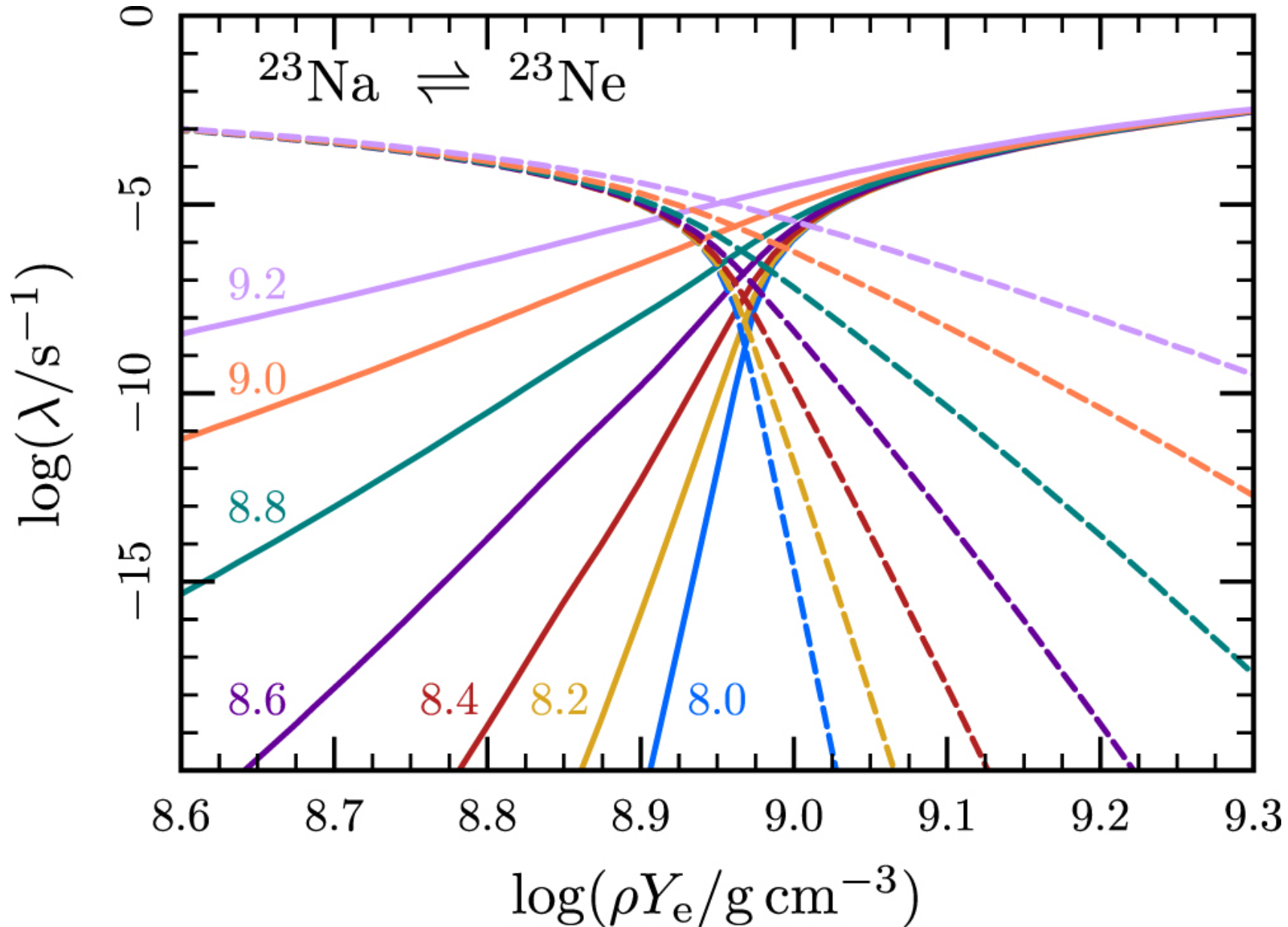
Figure 35. from MODULES FOR EXPERIMENTS IN STELLAR ASTROPHYSICS (MESA): BINARIES, PULSATIONS, AND EXPLOSIONS null 2015 APJS 220 15 doi:10.1088/0067-0049/220/1/15 https://dx.doi.org/10.1088/0067-0049/220/1/15 © 2015. The American Astronomical Society. All rights reserved.
