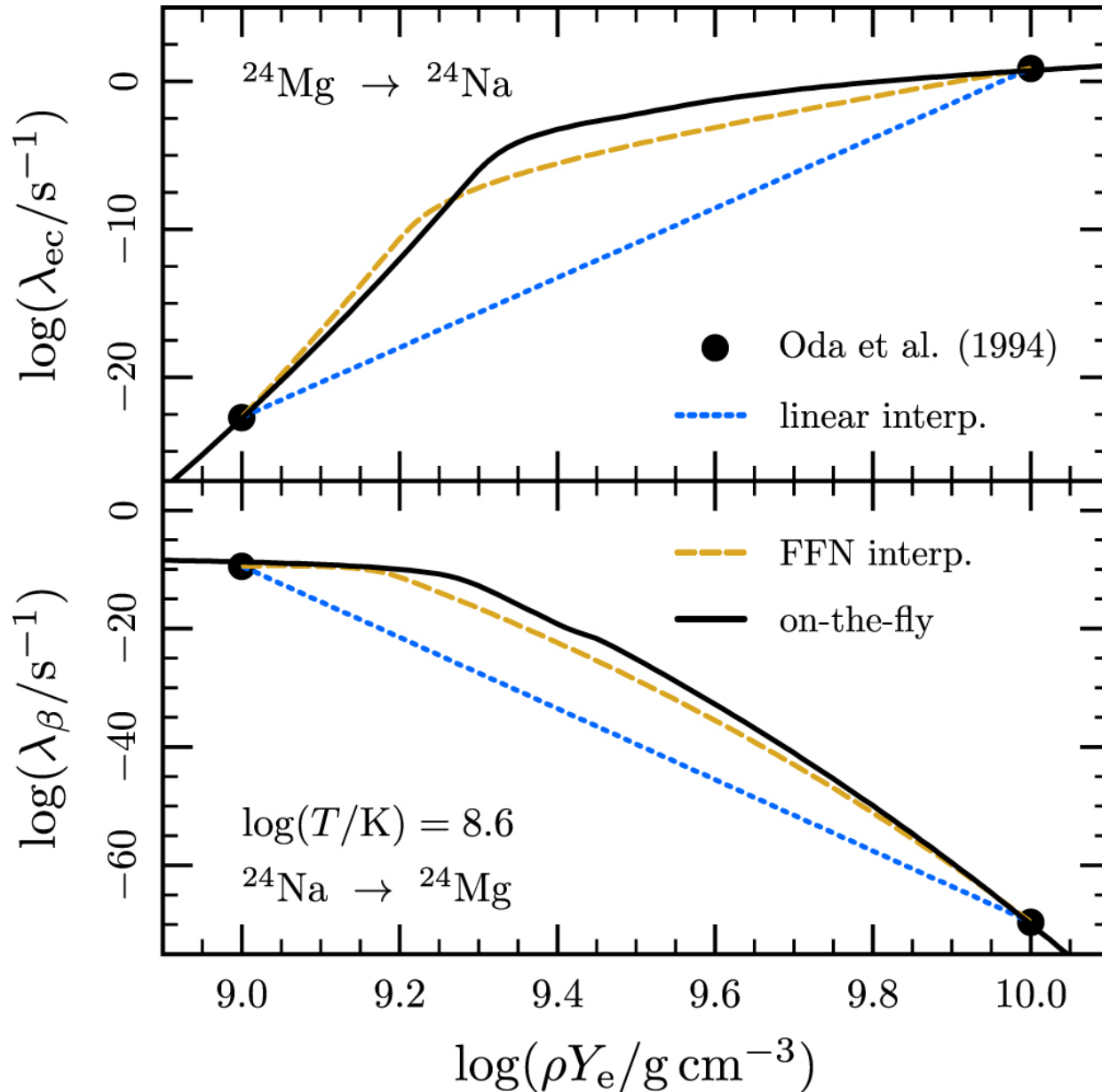
Figure 34. from MODULES FOR EXPERIMENTS IN STELLAR ASTROPHYSICS (MESA): BINARIES, PULSATIONS, AND EXPLOSIONS null 2015 APJS 220 15 doi:10.1088/0067-0049/220/1/15 https://dx.doi.org/10.1088/0067-0049/220/1/15 © 2015. The American Astronomical Society. All rights reserved.
