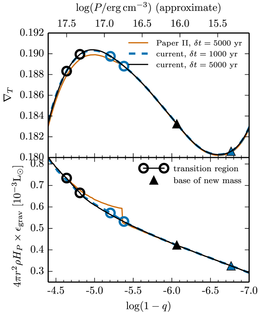
Figure 33. from MODULES FOR EXPERIMENTS IN STELLAR ASTROPHYSICS (MESA): BINARIES, PULSATIONS, AND EXPLOSIONS null 2015 APJS 220 15 doi:10.1088/0067-0049/220/1/15 https://dx.doi.org/10.1088/0067-0049/220/1/15 © 2015. The American Astronomical Society. All rights reserved.
